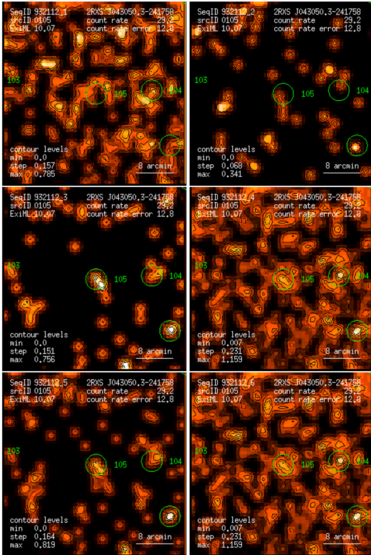
Figure 105: RASS 932112: detection 0105: band rate images, Gaussian filter: (1) PSPC channels 11 – 41, (2) 52 – 90, (3) 91 – 201, (4) 11 – 235, (5) 52 – 201, (6) 11 – 201. Broad band rates in counts/ks. Band rate contour levels in counts/ks/arcmin 2 .
