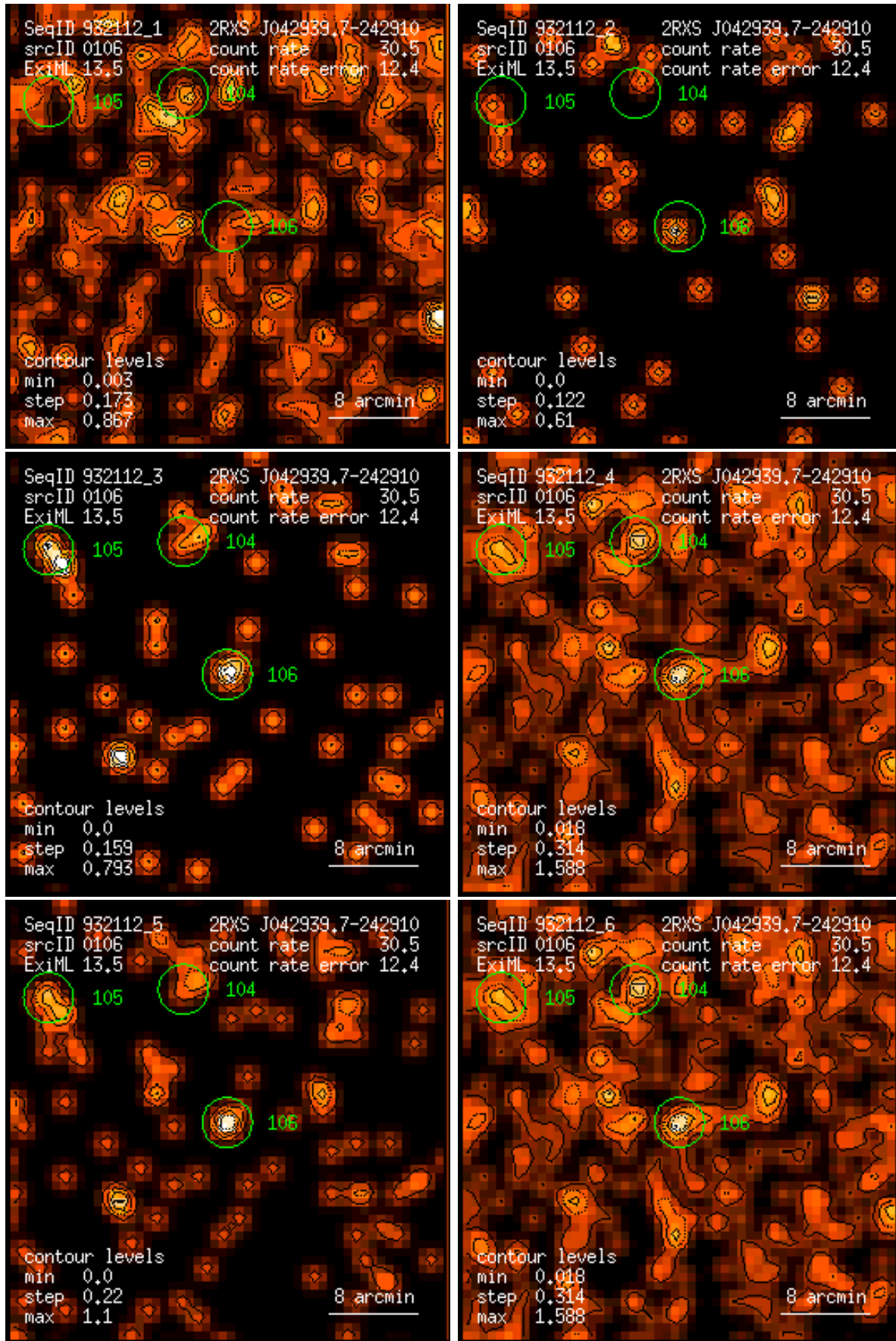
Figure 106: RASS 932112: detection 0106: band rate images, Gaussian filter: (1) PSPC channels 11 – 41, (2) 52 – 90, (3) 91 – 201, (4) 11 – 235, (5) 52 – 201, (6) 11 – 201. Broad band rates in counts/ks. Band rate contour levels in counts/ks/arcmin 2 .
