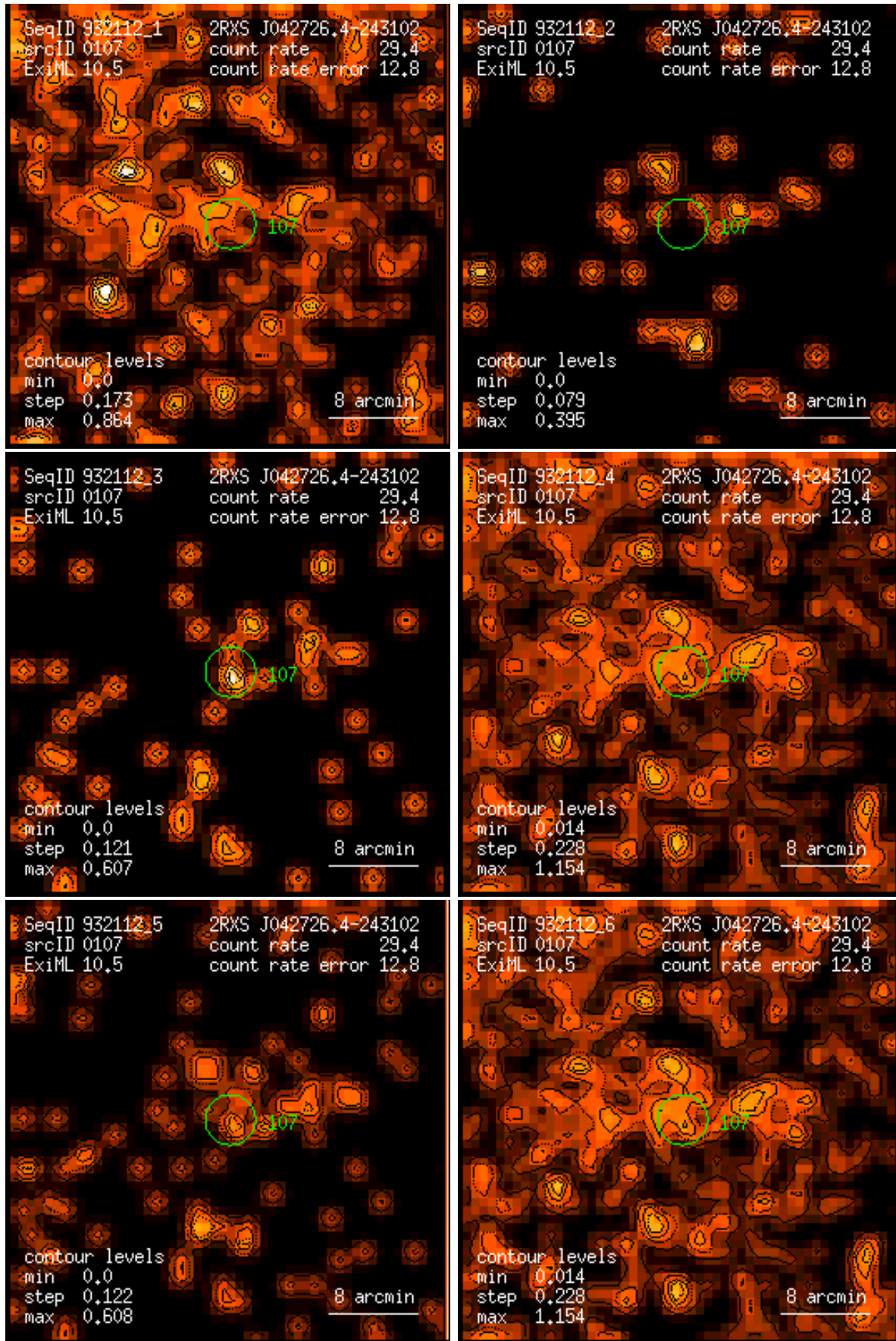
Figure 107: RASS 932112: detection 0107: band rate images, Gaussian filter: (1) PSPC channels 11 – 41, (2) 52 – 90, (3) 91 – 201, (4) 11 – 235, (5) 52 – 201, (6) 11 – 201. Broad band rates in counts/ks. Band rate contour levels in counts/ks/arcmin 2 .
