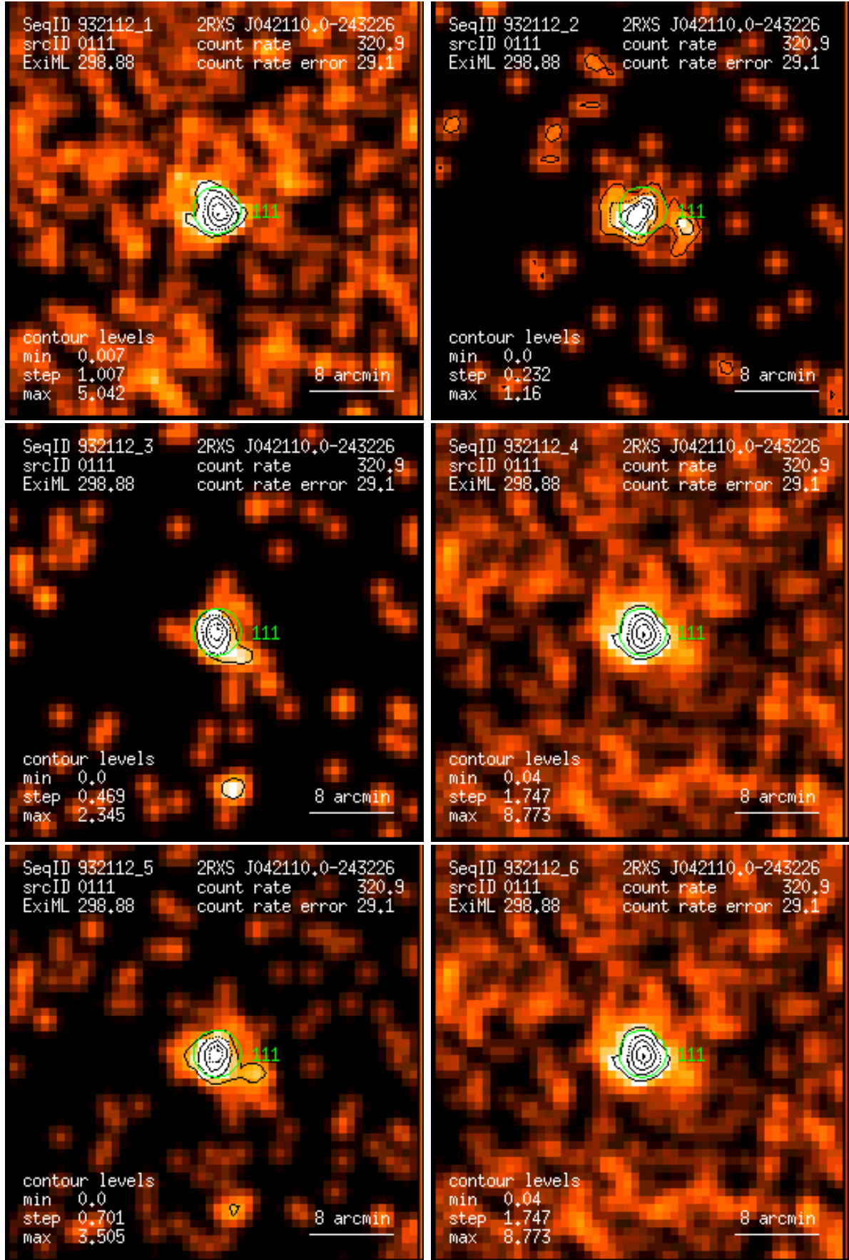
Figure 111: RASS 932112: detection 0111: band rate images, Gaussian filter: (1) PSPC channels 11 – 41, (2) 52 – 90, (3) 91 – 201, (4) 11 – 235, (5) 52 – 201, (6) 11 – 201. Broad band rates in counts/ks. Band rate contour levels in counts/ks/arcmin 2 .
