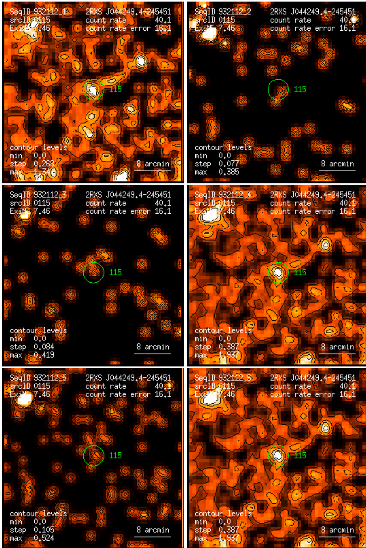
Figure 115: RASS 932112: detection 0115: band rate images, Gaussian filter: (1) PSPC channels 11 – 41, (2) 52 – 90, (3) 91 – 201, (4) 11 – 235, (5) 52 – 201, (6) 11 – 201. Broad band rates in counts/ks. Band rate contour levels in counts/ks/arcmin 2 .
