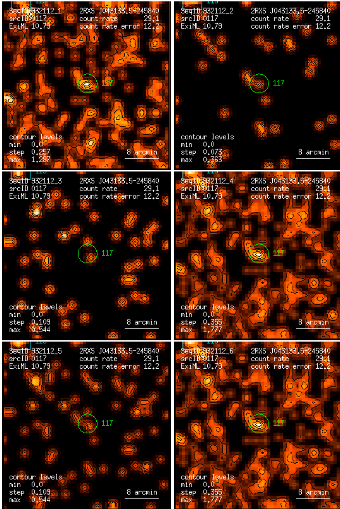
Figure 117: RASS 932112: detection 0117: band rate images, Gaussian filter: (1) PSPC channels 11 – 41, (2) 52 – 90, (3) 91 – 201, (4) 11 – 235, (5) 52 – 201, (6) 11 – 201. Broad band rates in counts/ks. Band rate contour levels in counts/ks/arcmin 2 .
