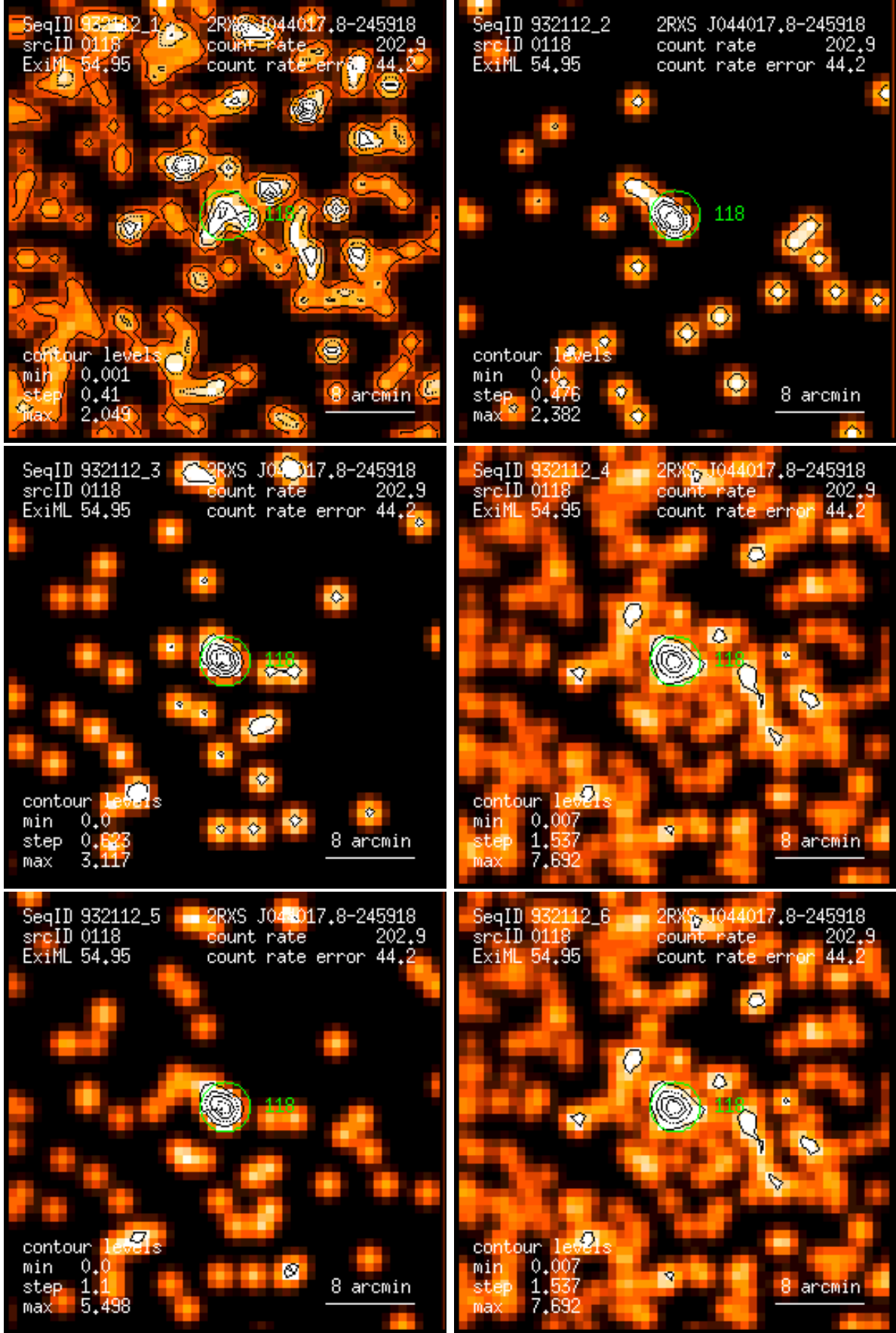
Figure 118: RASS 932112: detection 0118: band rate images, Gaussian filter: (1) PSPC channels 11 – 41, (2) 52 – 90, (3) 91 – 201, (4) 11 – 235, (5) 52 – 201, (6) 11 – 201. Broad band rates in counts/ks. Band rate contour levels in counts/ks/arcmin 2 .
