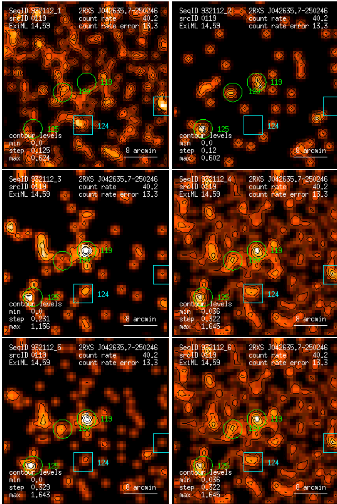
Figure 119: RASS 932112: detection 0119: band rate images, Gaussian filter: (1) PSPC channels 11 – 41, (2) 52 – 90, (3) 91 – 201, (4) 11 – 235, (5) 52 – 201, (6) 11 – 201. Broad band rates in counts/ks. Band rate contour levels in counts/ks/arcmin 2 .
