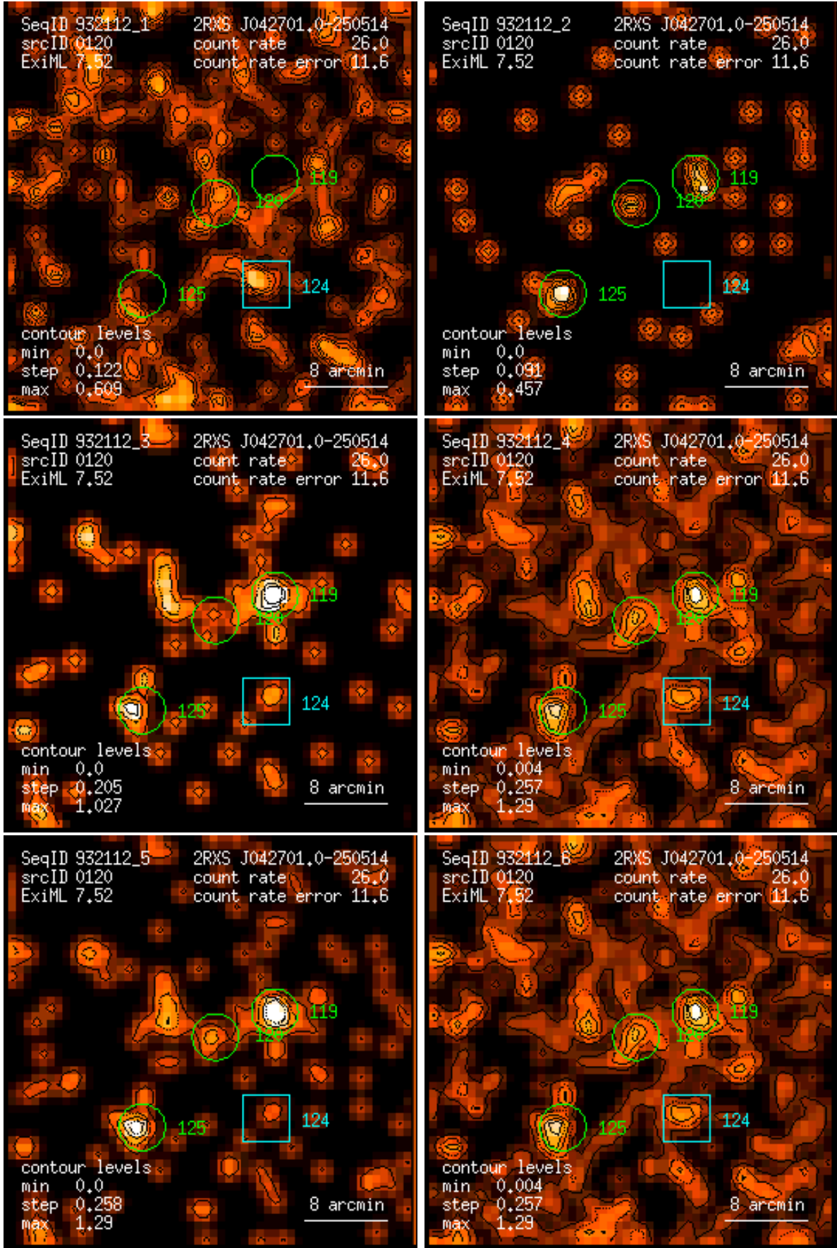
Figure 120: RASS 932112: detection 0120: band rate images, Gaussian filter: (1) PSPC channels 11 – 41, (2) 52 – 90, (3) 91 – 201, (4) 11 – 235, (5) 52 – 201, (6) 11 – 201. Broad band rates in counts/ks. Band rate contour levels in counts/ks/arcmin 2 .
