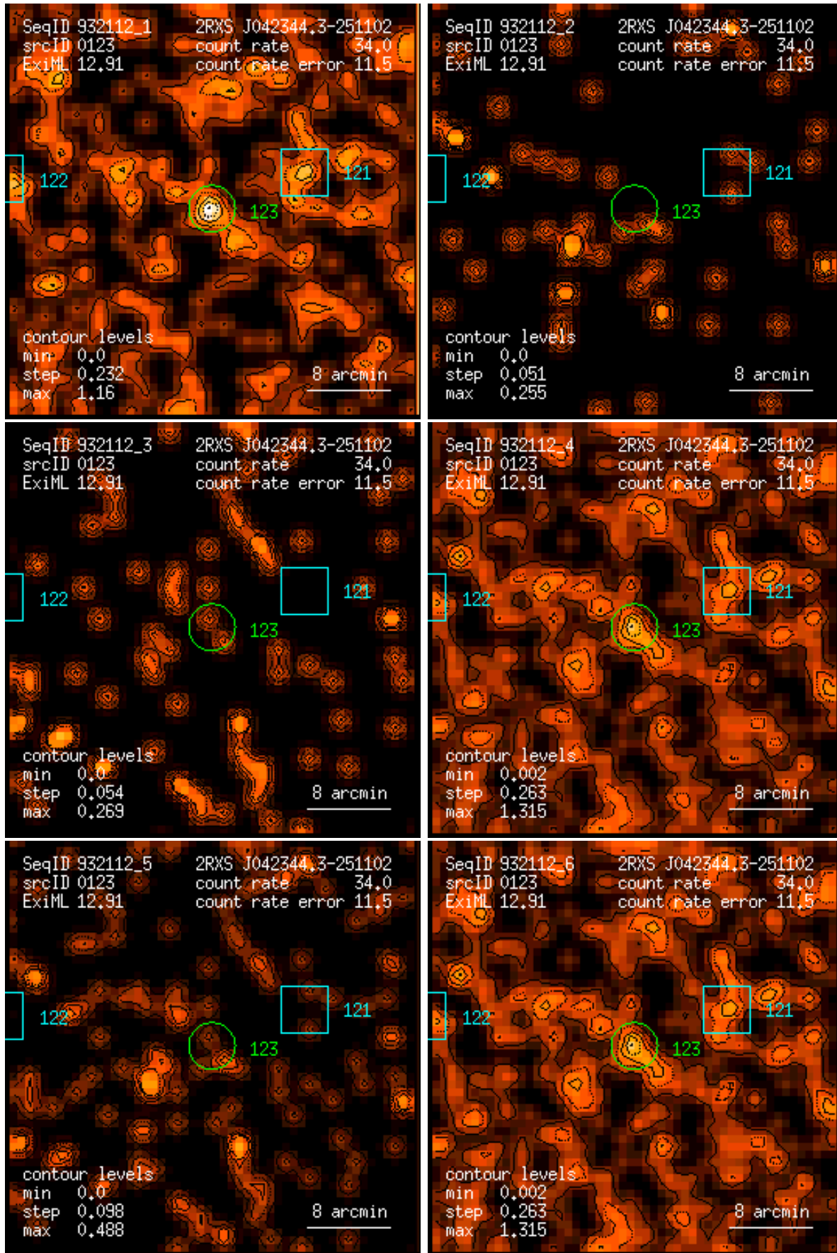
Figure 123: RASS 932112: detection 0123: band rate images, Gaussian filter: (1) PSPC channels 11 – 41, (2) 52 – 90, (3) 91 – 201, (4) 11 – 235, (5) 52 – 201, (6) 11 – 201. Broad band rates in counts/ks. Band rate contour levels in counts/ks/arcmin 2 .
