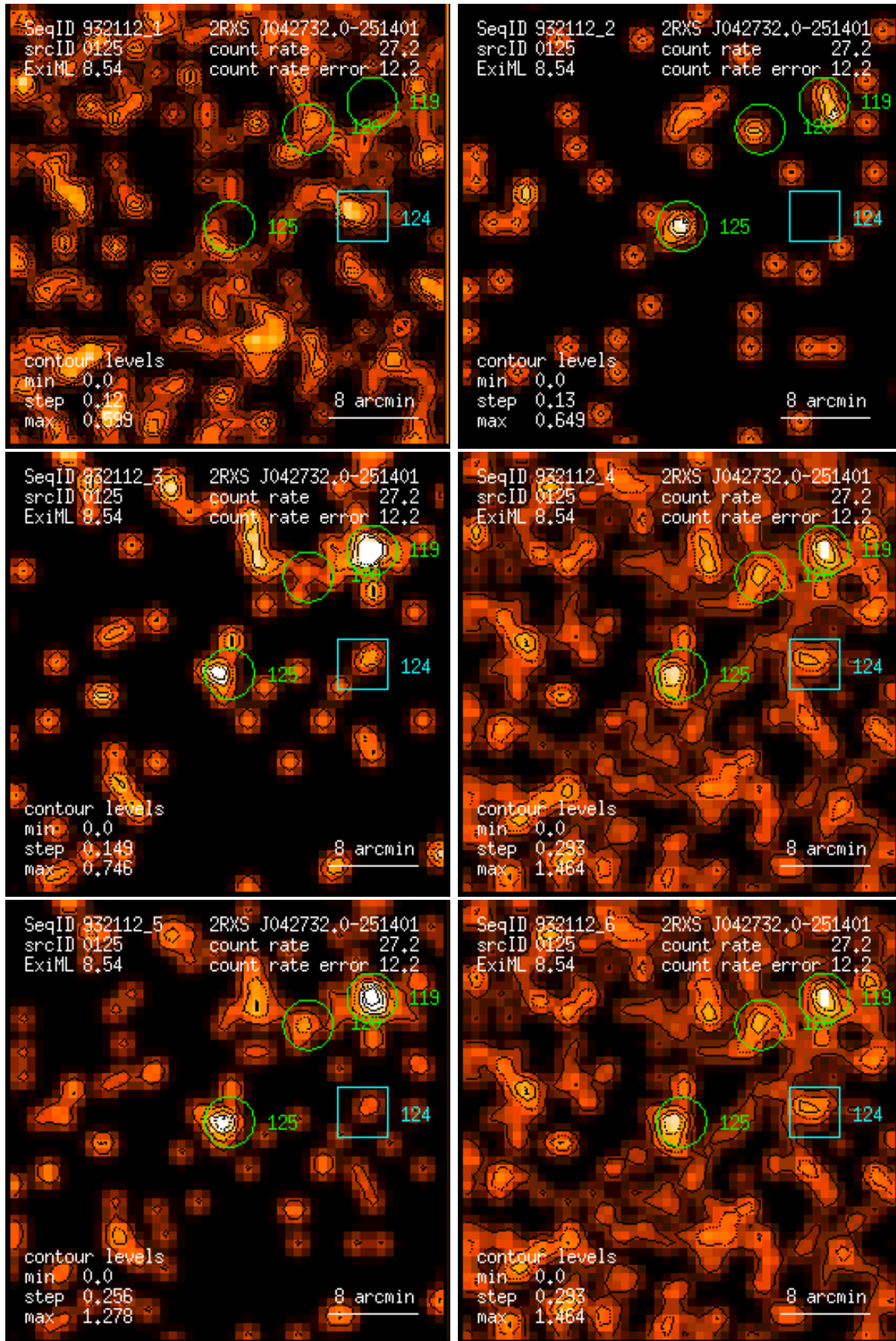
Figure 125: RASS 932112: detection 0125: band rate images, Gaussian filter: (1) PSPC channels 11 – 41, (2) 52 – 90, (3) 91 – 201, (4) 11 – 235, (5) 52 – 201, (6) 11 – 201. Broad band rates in counts/ks. Band rate contour levels in counts/ks/arcmin 2 .
