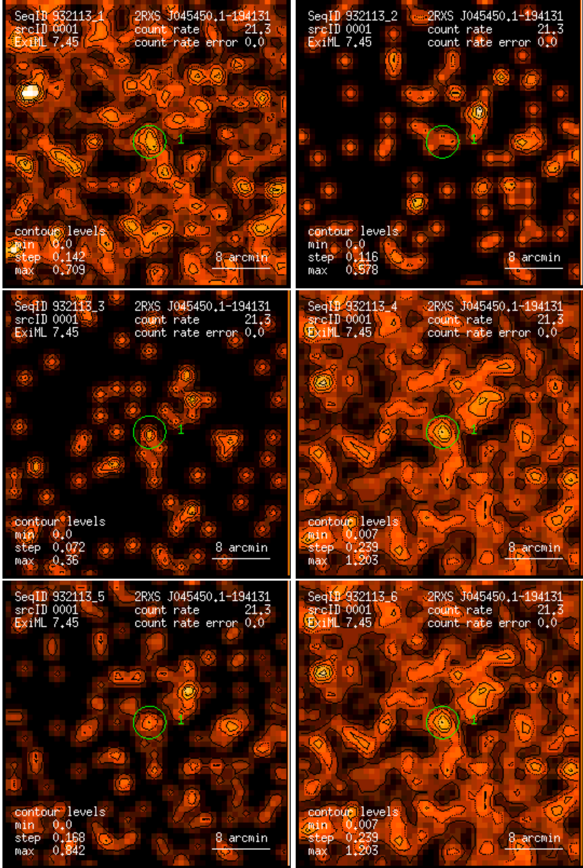
Figure 1: RASS 932113: detection 0001: band rate images, Gaussian filter: (1) PSPC channels 11 – 41, (2) 52 – 90, (3) 91 – 201, (4) 11 – 235, (5) 52 – 201, (6) 11 – 201. Broad band rates in counts/ks. Band rate contour levels in counts/ks/arcmin 2 .
