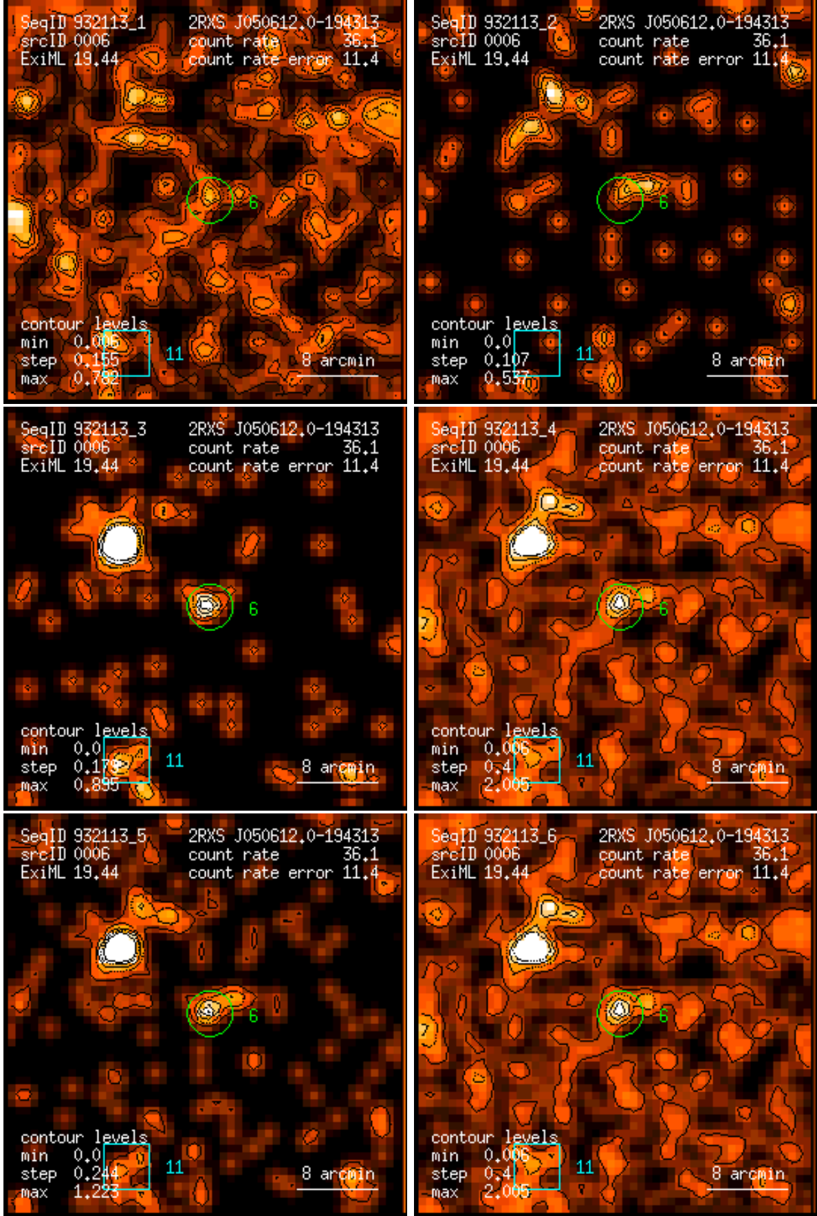
Figure 6: RASS 932113: detection 0006: band rate images, Gaussian filter: (1) PSPC channels 11 – 41, (2) 52 – 90, (3) 91 – 201, (4) 11 – 235, (5) 52 – 201, (6) 11 – 201. Broad band rates in counts/ks. Band rate contour levels in counts/ks/arcmin 2 .
