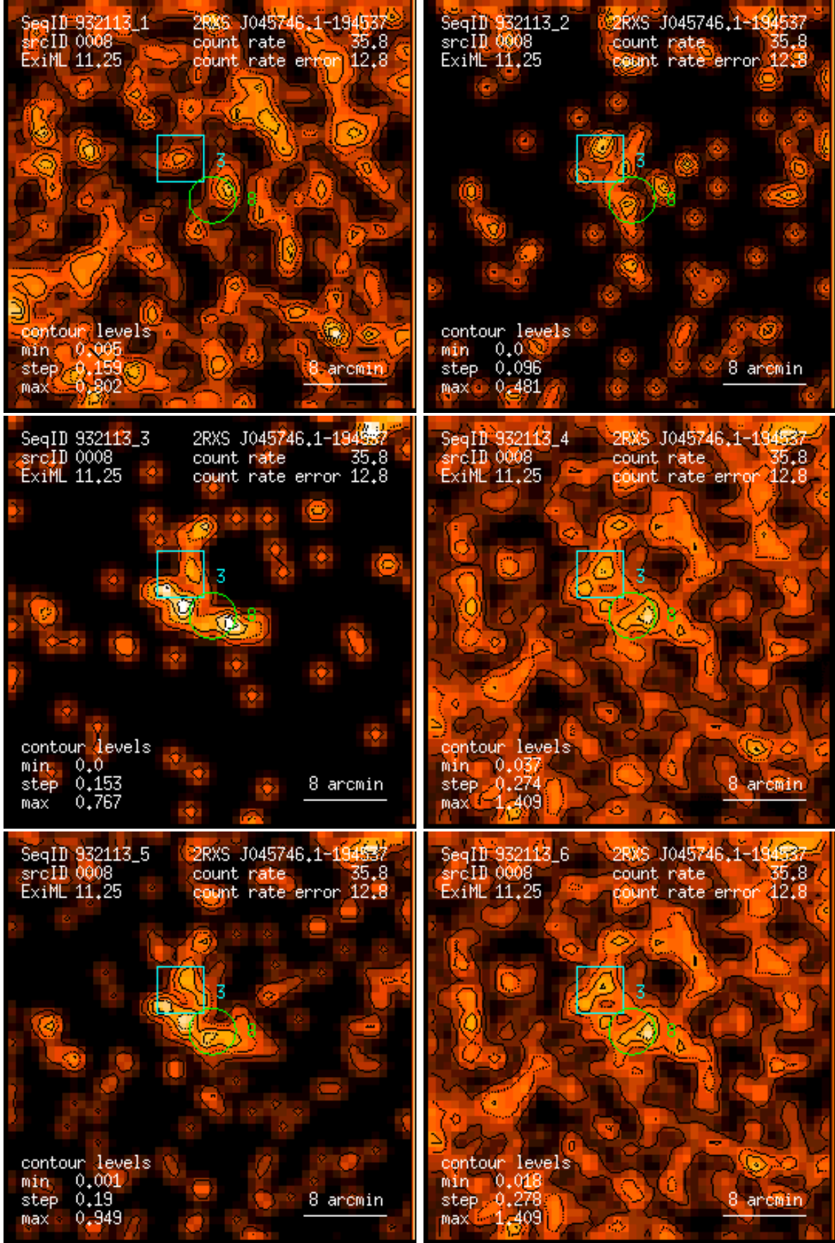
Figure 8: RASS 932113: detection 0008: band rate images, Gaussian filter: (1) PSPC channels 11 – 41, (2) 52 – 90, (3) 91 – 201, (4) 11 – 235, (5) 52 – 201, (6) 11 – 201. Broad band rates in counts/ks. Band rate contour levels in counts/ks/arcmin 2 .
