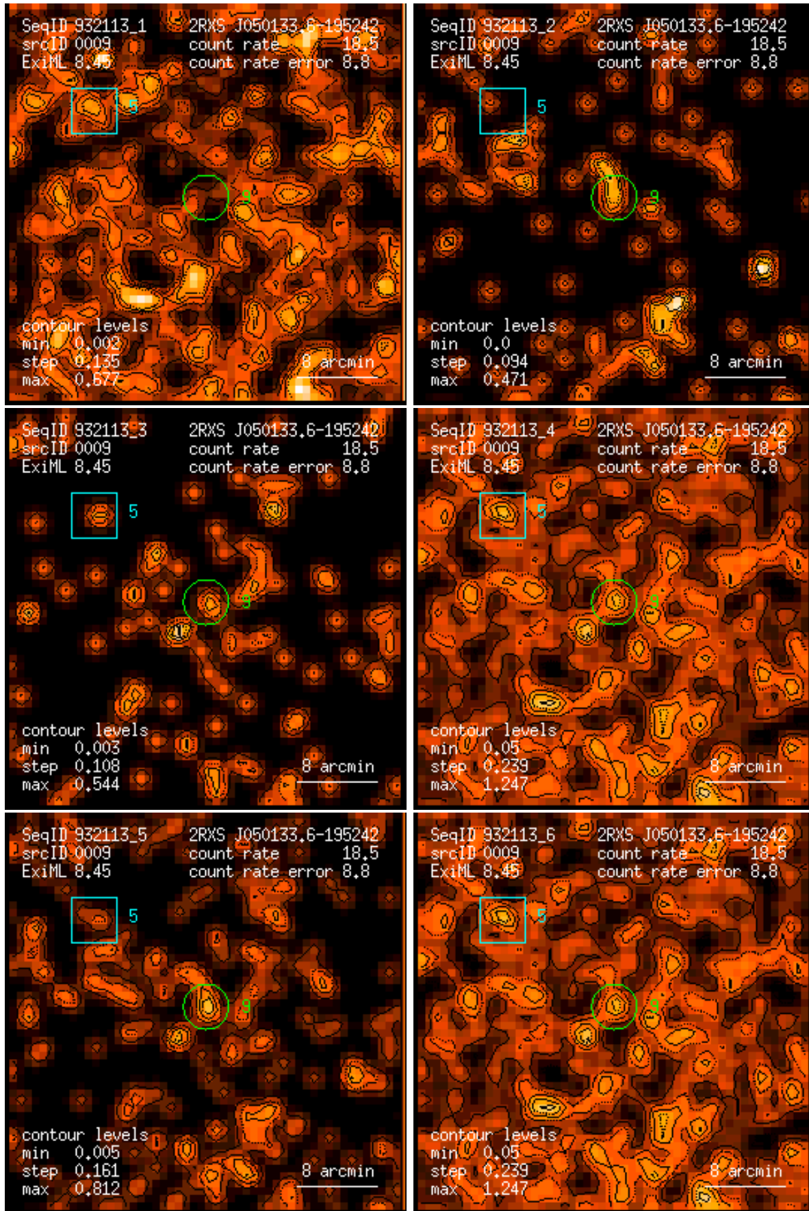
Figure 9: RASS 932113: detection 0009: band rate images, Gaussian filter: (1) PSPC channels 11 – 41, (2) 52 – 90, (3) 91 – 201, (4) 11 – 235, (5) 52 – 201, (6) 11 – 201. Broad band rates in counts/ks. Band rate contour levels in counts/ks/arcmin 2 .
