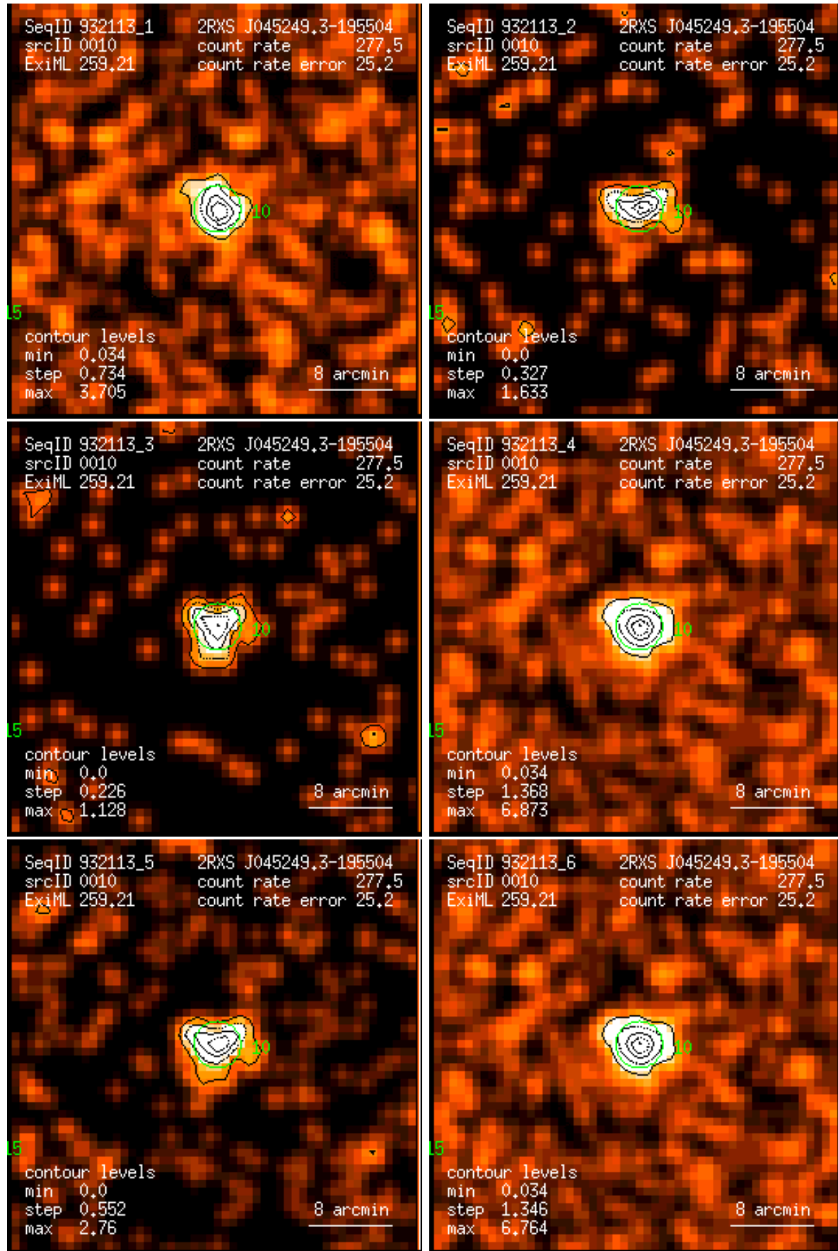
Figure 10: RASS 932113: detection 0010: band rate images, Gaussian filter: (1) PSPC channels 11 – 41, (2) 52 – 90, (3) 91 – 201, (4) 11 – 235, (5) 52 – 201, (6) 11 – 201. Broad band rates in counts/ks. Band rate contour levels in counts/ks/arcmin 2 .
