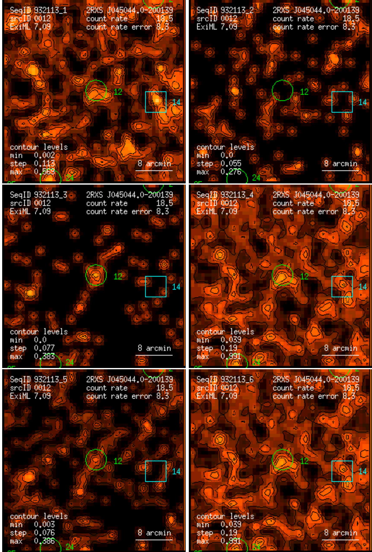
Figure 12: RASS 932113: detection 0012: band rate images, Gaussian filter: (1) PSPC channels 11 – 41, (2) 52 – 90, (3) 91 – 201, (4) 11 – 235, (5) 52 – 201, (6) 11 – 201. Broad band rates in counts/ks. Band rate contour levels in counts/ks/arcmin 2 .
