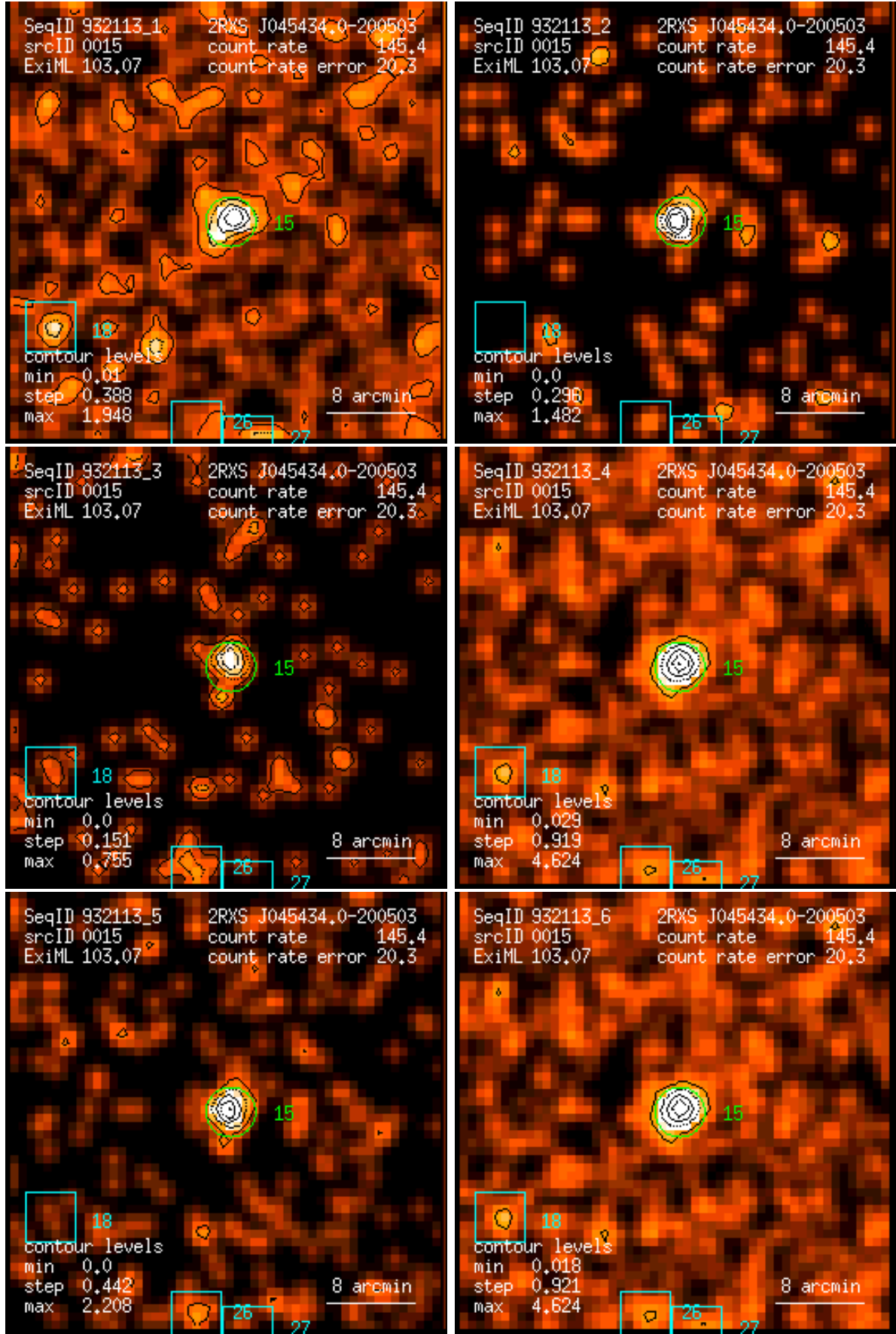
Figure 15: RASS 932113: detection 0015: band rate images, Gaussian filter: (1) PSPC channels 11 – 41, (2) 52 – 90, (3) 91 – 201, (4) 11 – 235, (5) 52 – 201, (6) 11 – 201. Broad band rates in counts/ks. Band rate contour levels in counts/ks/arcmin 2 .
