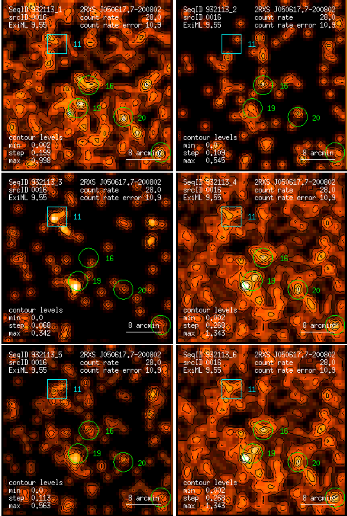
Figure 16: RASS 932113: detection 0016: band rate images, Gaussian filter: (1) PSPC channels 11 – 41, (2) 52 – 90, (3) 91 – 201, (4) 11 – 235, (5) 52 – 201, (6) 11 – 201. Broad band rates in counts/ks. Band rate contour levels in counts/ks/arcmin 2 .
