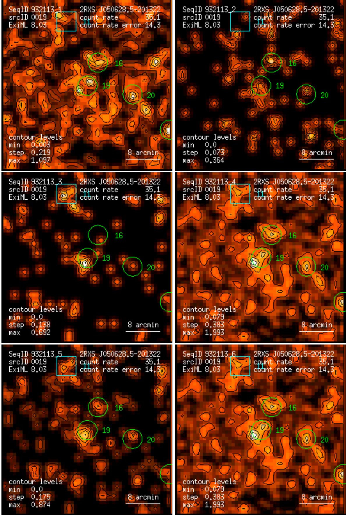
Figure 19: RASS 932113: detection 0019: band rate images, Gaussian filter: (1) PSPC channels 11 – 41, (2) 52 – 90, (3) 91 – 201, (4) 11 – 235, (5) 52 – 201, (6) 11 – 201. Broad band rates in counts/ks. Band rate contour levels in counts/ks/arcmin 2 .
