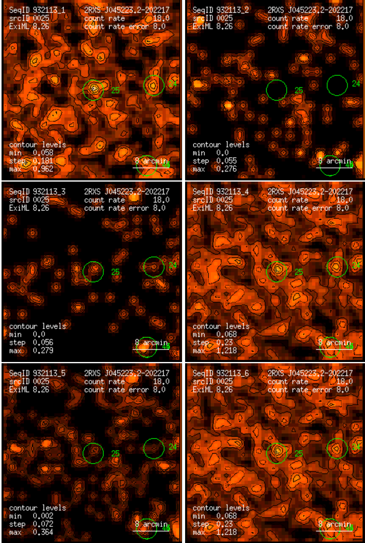
Figure 25: RASS 932113: detection 0025: band rate images, Gaussian filter: (1) PSPC channels 11 – 41, (2) 52 – 90, (3) 91 – 201, (4) 11 – 235, (5) 52 – 201, (6) 11 – 201. Broad band rates in counts/ks. Band rate contour levels in counts/ks/arcmin 2 .
