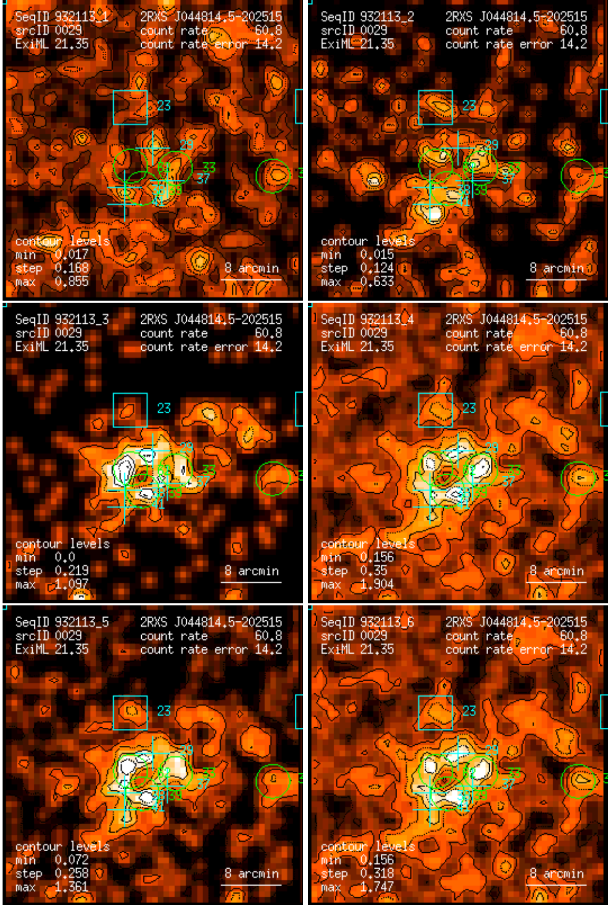
Figure 29: RASS 932113: detection 0029: band rate images, Gaussian filter: (1) PSPC channels 11 – 41, (2) 52 – 90, (3) 91 – 201, (4) 11 – 235, (5) 52 – 201, (6) 11 – 201. Broad band rates in counts/ks. Band rate contour levels in counts/ks/arcmin 2 .
