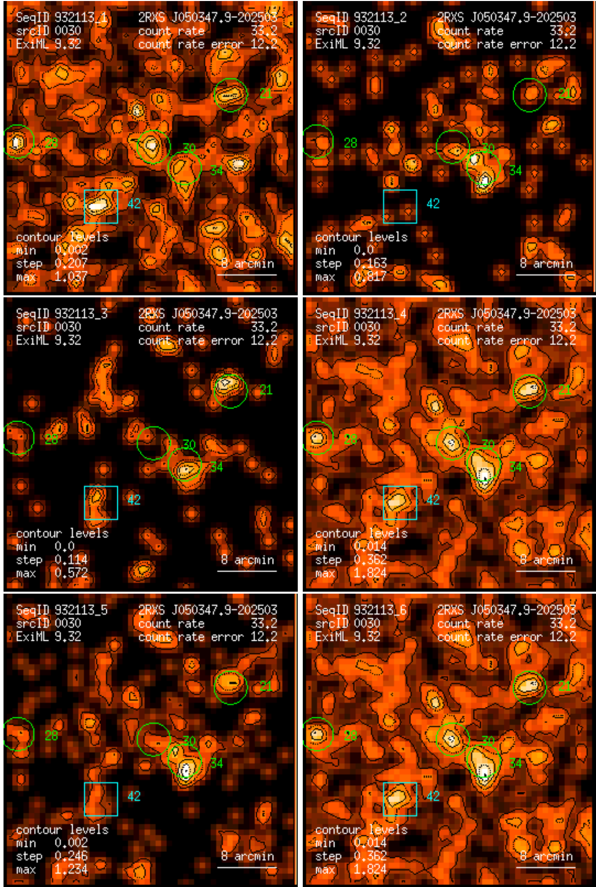
Figure 30: RASS 932113: detection 0030: band rate images, Gaussian filter: (1) PSPC channels 11 – 41, (2) 52 – 90, (3) 91 – 201, (4) 11 – 235, (5) 52 – 201, (6) 11 – 201. Broad band rates in counts/ks. Band rate contour levels in counts/ks/arcmin 2 .
