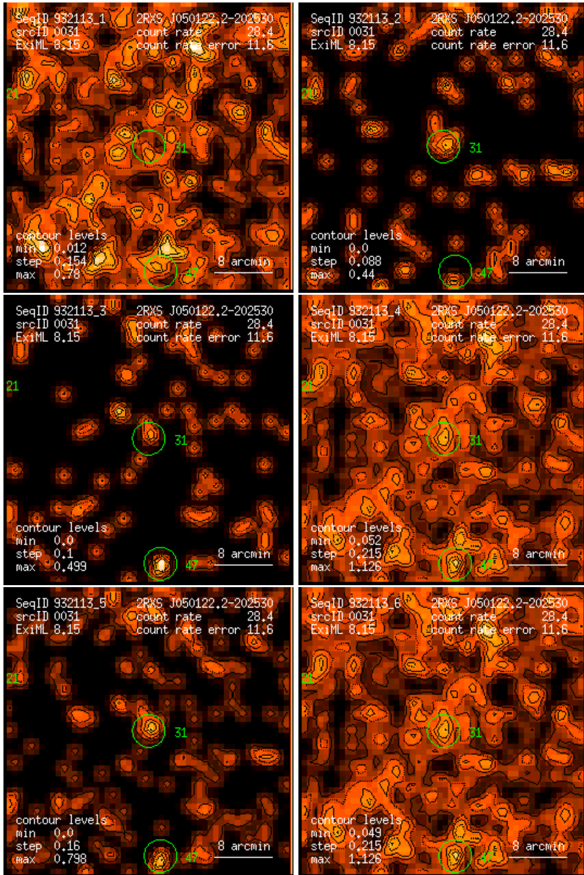
Figure 31: RASS 932113: detection 0031: band rate images, Gaussian filter: (1) PSPC channels 11 – 41, (2) 52 – 90, (3) 91 – 201, (4) 11 – 235, (5) 52 – 201, (6) 11 – 201. Broad band rates in counts/ks. Band rate contour levels in counts/ks/arcmin 2 .
