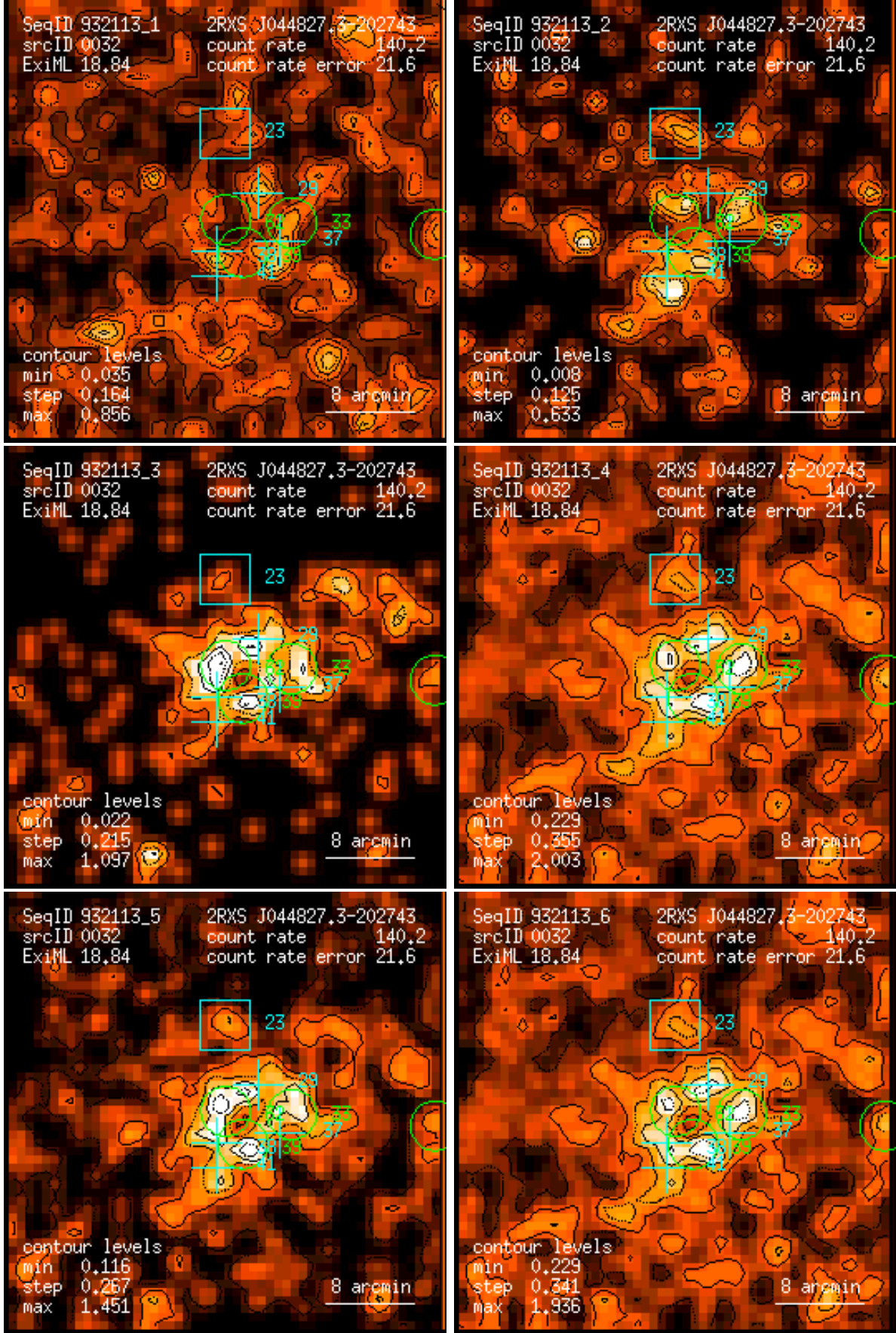
Figure 32: RASS 932113: detection 0032: band rate images, Gaussian filter: (1) PSPC channels 11 – 41, (2) 52 – 90, (3) 91 – 201, (4) 11 – 235, (5) 52 – 201, (6) 11 – 201. Broad band rates in counts/ks. Band rate contour levels in counts/ks/arcmin 2 .
