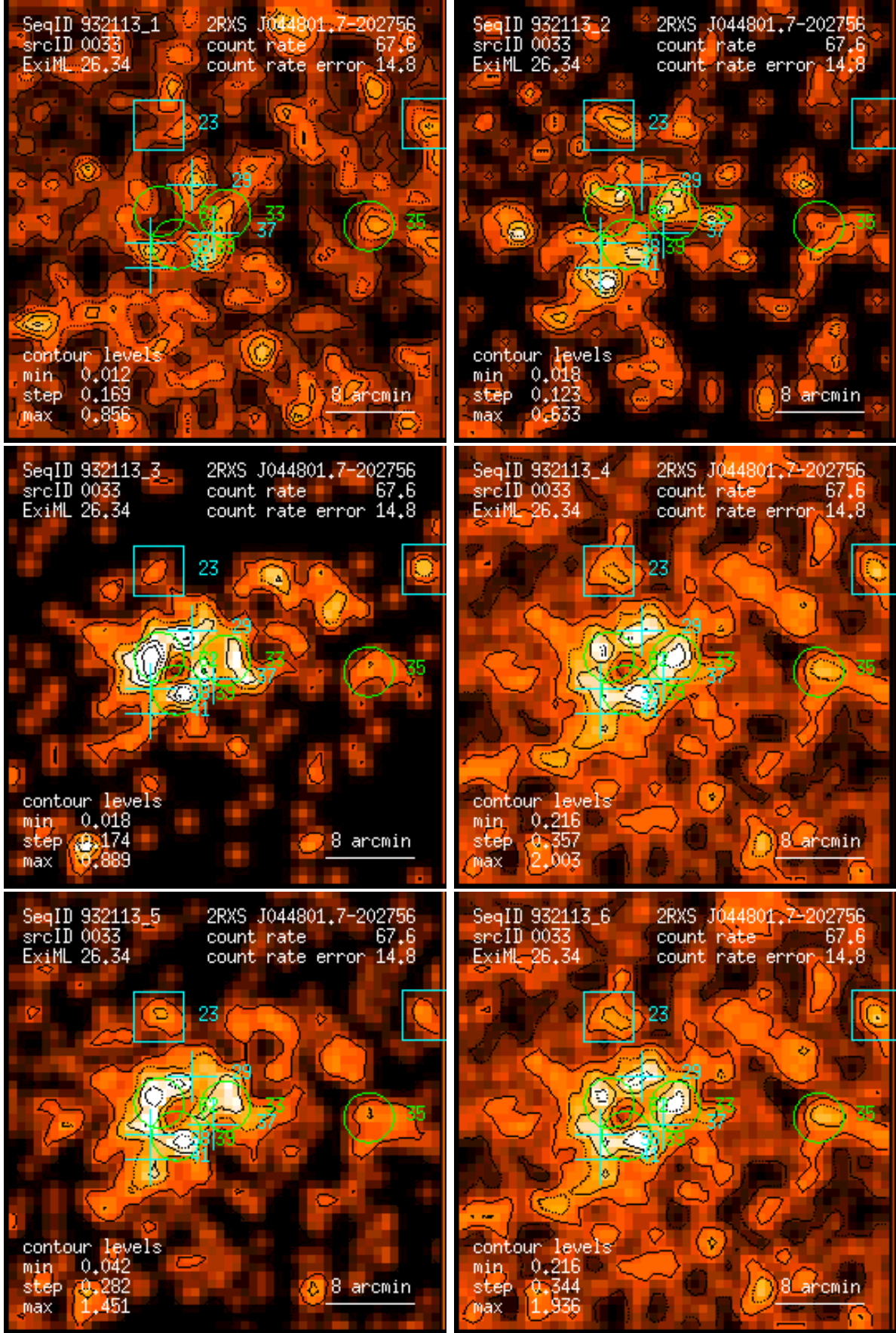
Figure 33: RASS 932113: detection 0033: band rate images, Gaussian filter: (1) PSPC channels 11 – 41, (2) 52 – 90, (3) 91 – 201, (4) 11 – 235, (5) 52 – 201, (6) 11 – 201. Broad band rates in counts/ks. Band rate contour levels in counts/ks/arcmin 2 .
