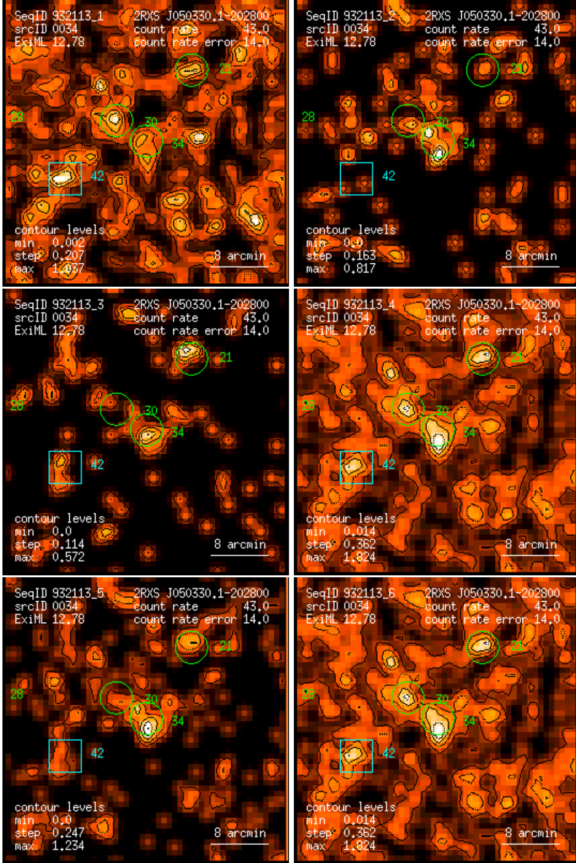
Figure 34: RASS 932113: detection 0034: band rate images, Gaussian filter: (1) PSPC channels 11 – 41, (2) 52 – 90, (3) 91 – 201, (4) 11 – 235, (5) 52 – 201, (6) 11 – 201. Broad band rates in counts/ks. Band rate contour levels in counts/ks/arcmin 2 .
