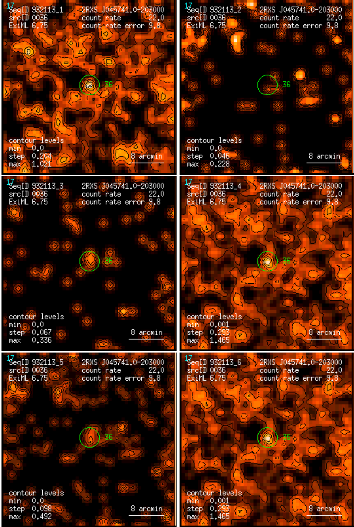
Figure 36: RASS 932113: detection 0036: band rate images, Gaussian filter: (1) PSPC channels 11 – 41, (2) 52 – 90, (3) 91 – 201, (4) 11 – 235, (5) 52 – 201, (6) 11 – 201. Broad band rates in counts/ks. Band rate contour levels in counts/ks/arcmin 2 .
