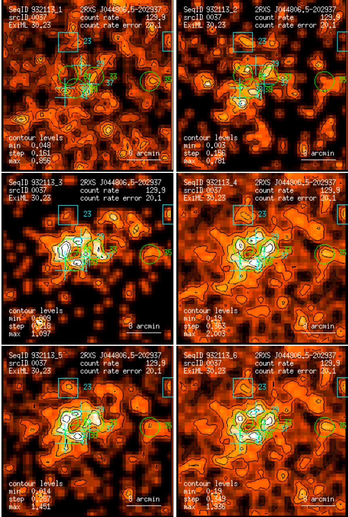
Figure 37: RASS 932113: detection 0037: band rate images, Gaussian filter: (1) PSPC channels 11 – 41, (2) 52 – 90, (3) 91 – 201, (4) 11 – 235, (5) 52 – 201, (6) 11 – 201. Broad band rates in counts/ks. Band rate contour levels in counts/ks/arcmin 2 .
