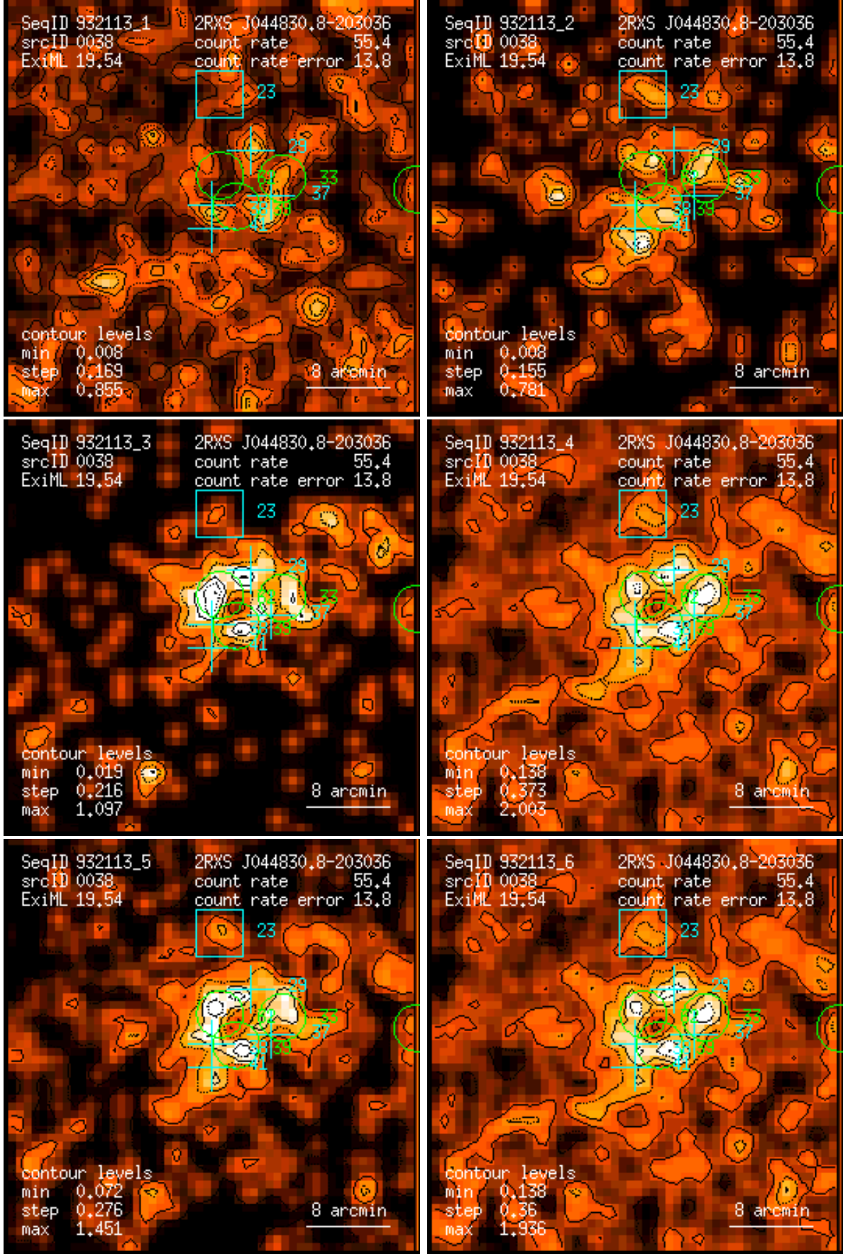
Figure 38: RASS 932113: detection 0038: band rate images, Gaussian filter: (1) PSPC channels 11 – 41, (2) 52 – 90, (3) 91 – 201, (4) 11 – 235, (5) 52 – 201, (6) 11 – 201. Broad band rates in counts/ks. Band rate contour levels in counts/ks/arcmin 2 .
