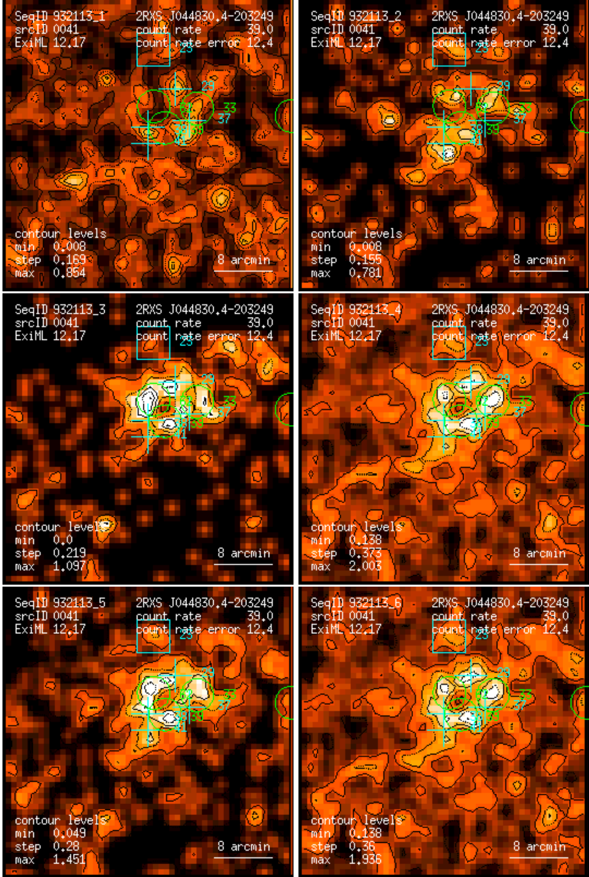
Figure 41: RASS 932113: detection 0041: band rate images, Gaussian filter: (1) PSPC channels 11 – 41, (2) 52 – 90, (3) 91 – 201, (4) 11 – 235, (5) 52 – 201, (6) 11 – 201. Broad band rates in counts/ks. Band rate contour levels in counts/ks/arcmin 2 .
