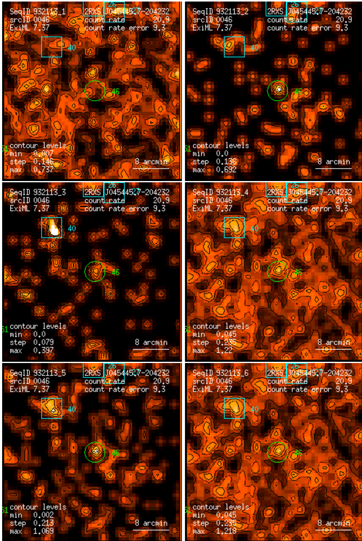
Figure 46: RASS 932113: detection 0046: band rate images, Gaussian filter: (1) PSPC channels 11 – 41, (2) 52 – 90, (3) 91 – 201, (4) 11 – 235, (5) 52 – 201, (6) 11 – 201. Broad band rates in counts/ks. Band rate contour levels in counts/ks/arcmin 2 .
