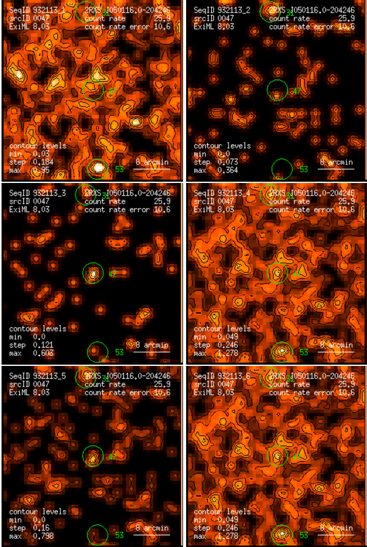
Figure 47: RASS 932113: detection 0047: band rate images, Gaussian filter: (1) PSPC channels 11 – 41, (2) 52 – 90, (3) 91 – 201, (4) 11 – 235, (5) 52 – 201, (6) 11 – 201. Broad band rates in counts/ks. Band rate contour levels in counts/ks/arcmin 2 .
