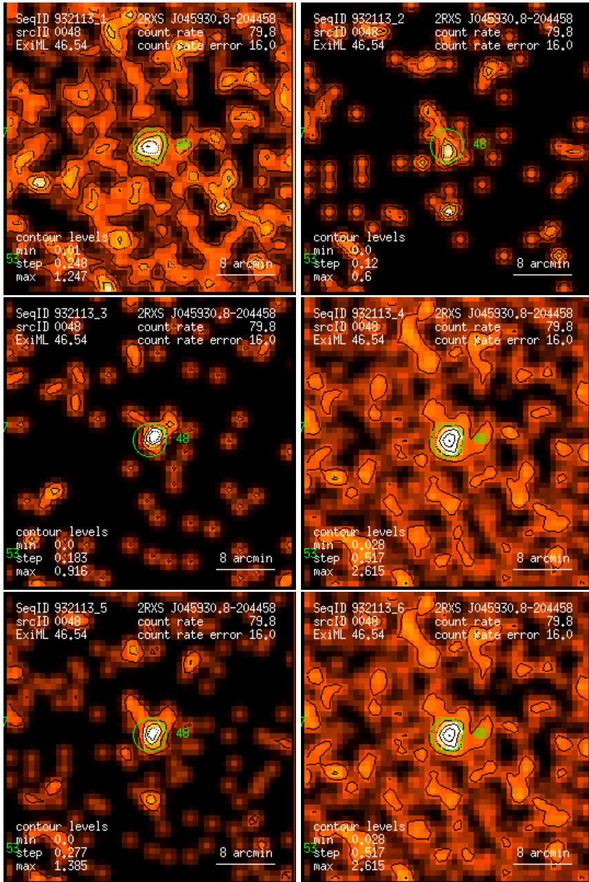
Figure 48: RASS 932113: detection 0048: band rate images, Gaussian filter: (1) PSPC channels 11 – 41, (2) 52 – 90, (3) 91 – 201, (4) 11 – 235, (5) 52 – 201, (6) 11 – 201. Broad band rates in counts/ks. Band rate contour levels in counts/ks/arcmin 2 .
