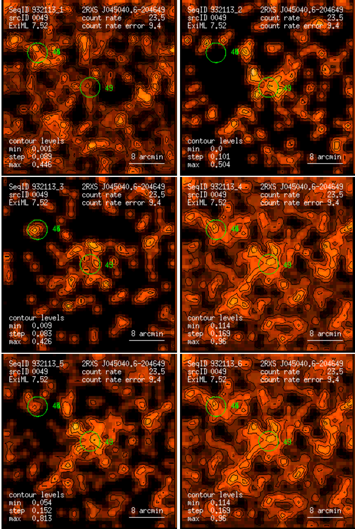
Figure 49: RASS 932113: detection 0049: band rate images, Gaussian filter: (1) PSPC channels 11 – 41, (2) 52 – 90, (3) 91 – 201, (4) 11 – 235, (5) 52 – 201, (6) 11 – 201. Broad band rates in counts/ks. Band rate contour levels in counts/ks/arcmin 2 .
