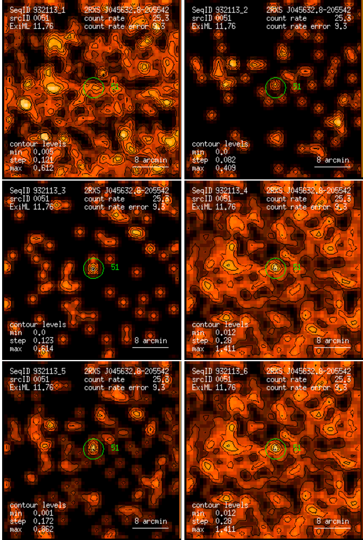
Figure 51: RASS 932113: detection 0051: band rate images, Gaussian filter: (1) PSPC channels 11 – 41, (2) 52 – 90, (3) 91 – 201, (4) 11 – 235, (5) 52 – 201, (6) 11 – 201. Broad band rates in counts/ks. Band rate contour levels in counts/ks/arcmin 2 .
