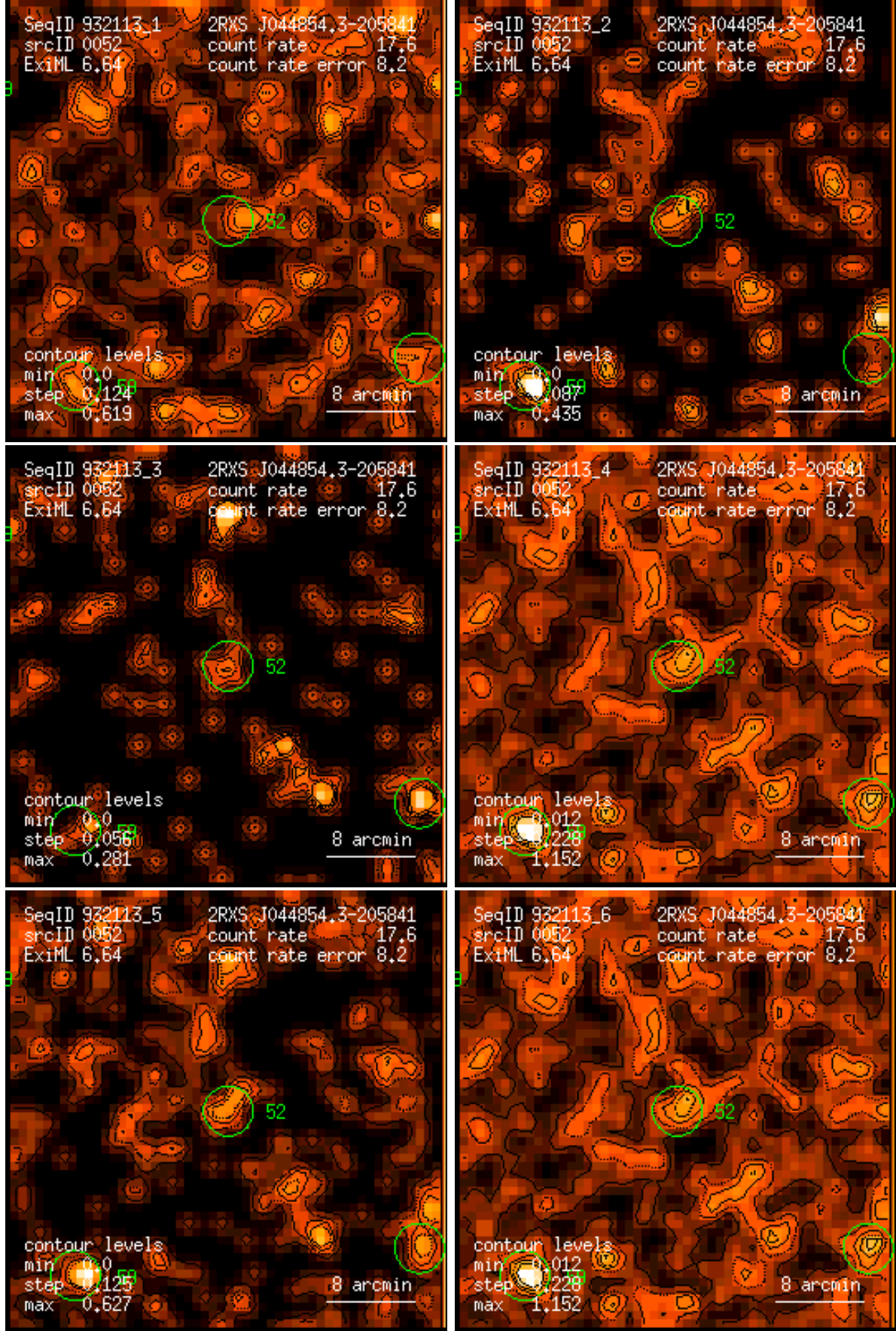
Figure 52: RASS 932113: detection 0052: band rate images, Gaussian filter: (1) PSPP channels 11 – 41, (2) 52 – 90, (3) 91 – 201, (4) 11 – 235, (5) 52 – 201, (6) 11 – 201. Broad band rates in counts/ks. Band rate contour levels in counts/ks/arcmin 2 .
