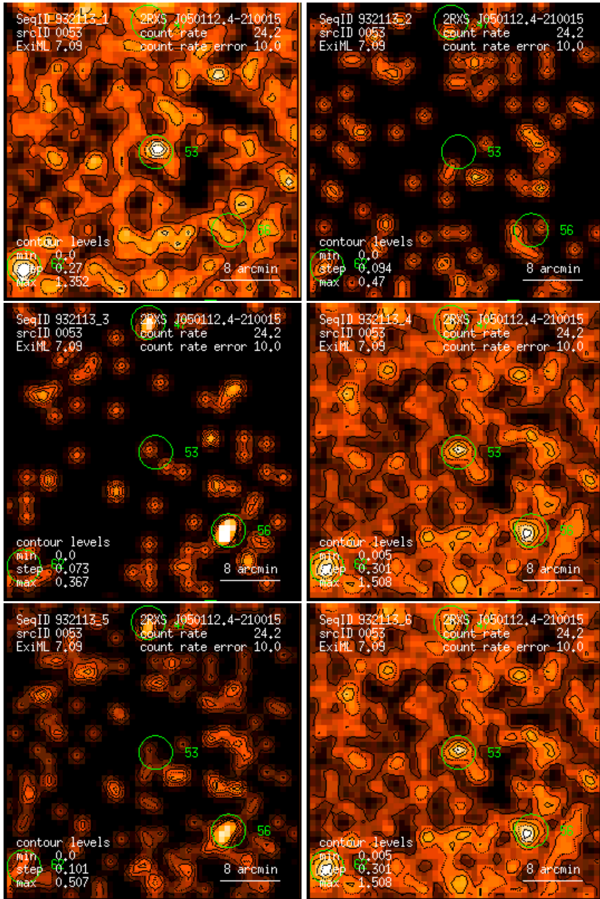
Figure 53: RASS 932113: detection 0053: band rate images, Gaussian filter: (1) PSPC channels 11 – 41, (2) 52 – 90, (3) 91 – 201, (4) 11 – 235, (5) 52 – 201, (6) 11 – 201. Broad band rates in counts/ks. Band rate contour levels in counts/ks/arcmin 2 .
