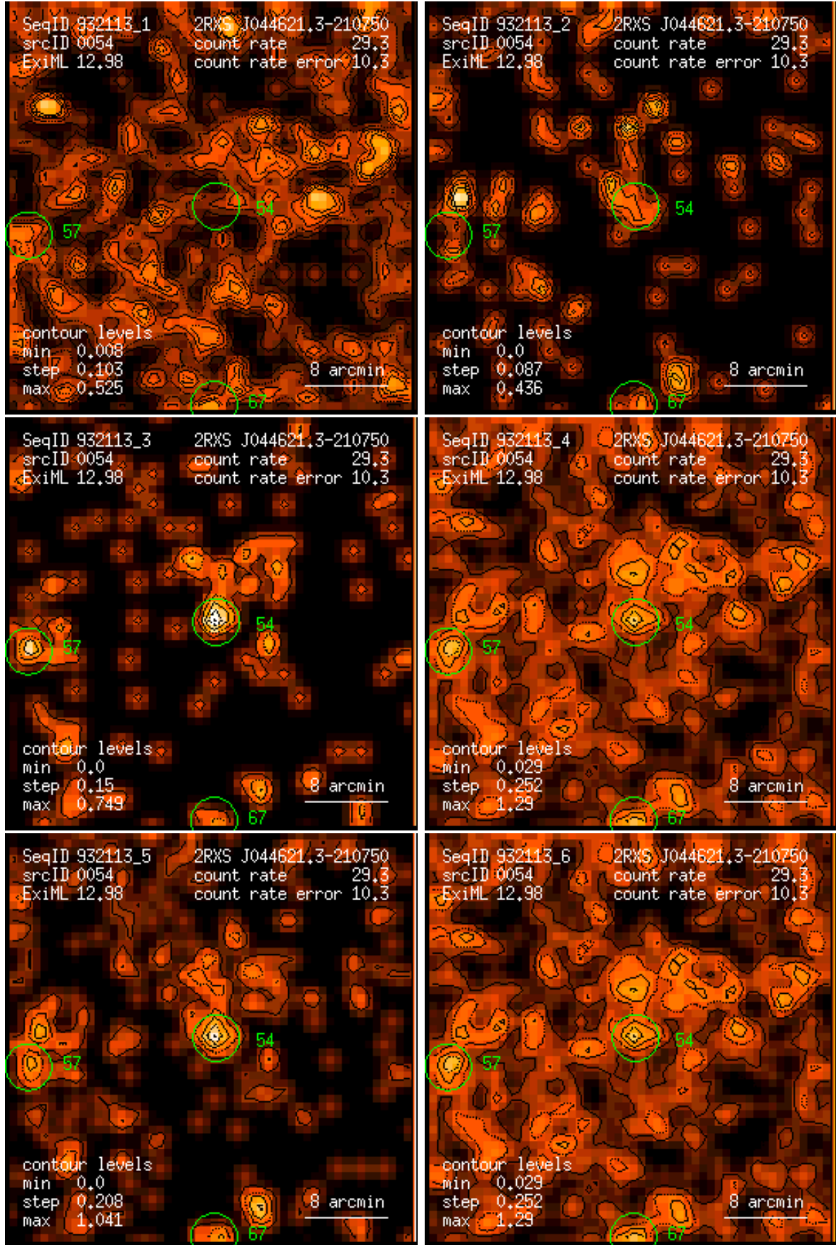
Figure 54: RASS 932113: detection 0054: band rate images, Gaussian filter: (1) PSPC channels 11 – 41, (2) 52 – 90, (3) 91 – 201, (4) 11 – 235, (5) 52 – 201, (6) 11 – 201. Broad band rates in counts/ks. Band rate contour levels in counts/ks/arcmin 2 .
