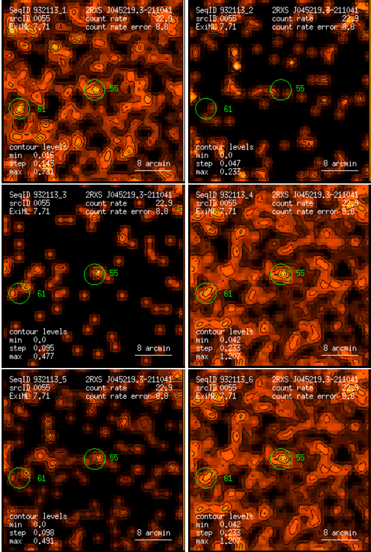
Figure 55: RASS 932113: detection 0055: band rate images, Gaussian filter: (1) PSPC channels 11 – 41, (2) 52 – 90, (3) 91 – 201, (4) 11 – 235, (5) 52 – 201, (6) 11 – 201. Broad band rates in counts/ks. Band rate contour levels in counts/ks/arcmin 2 .
