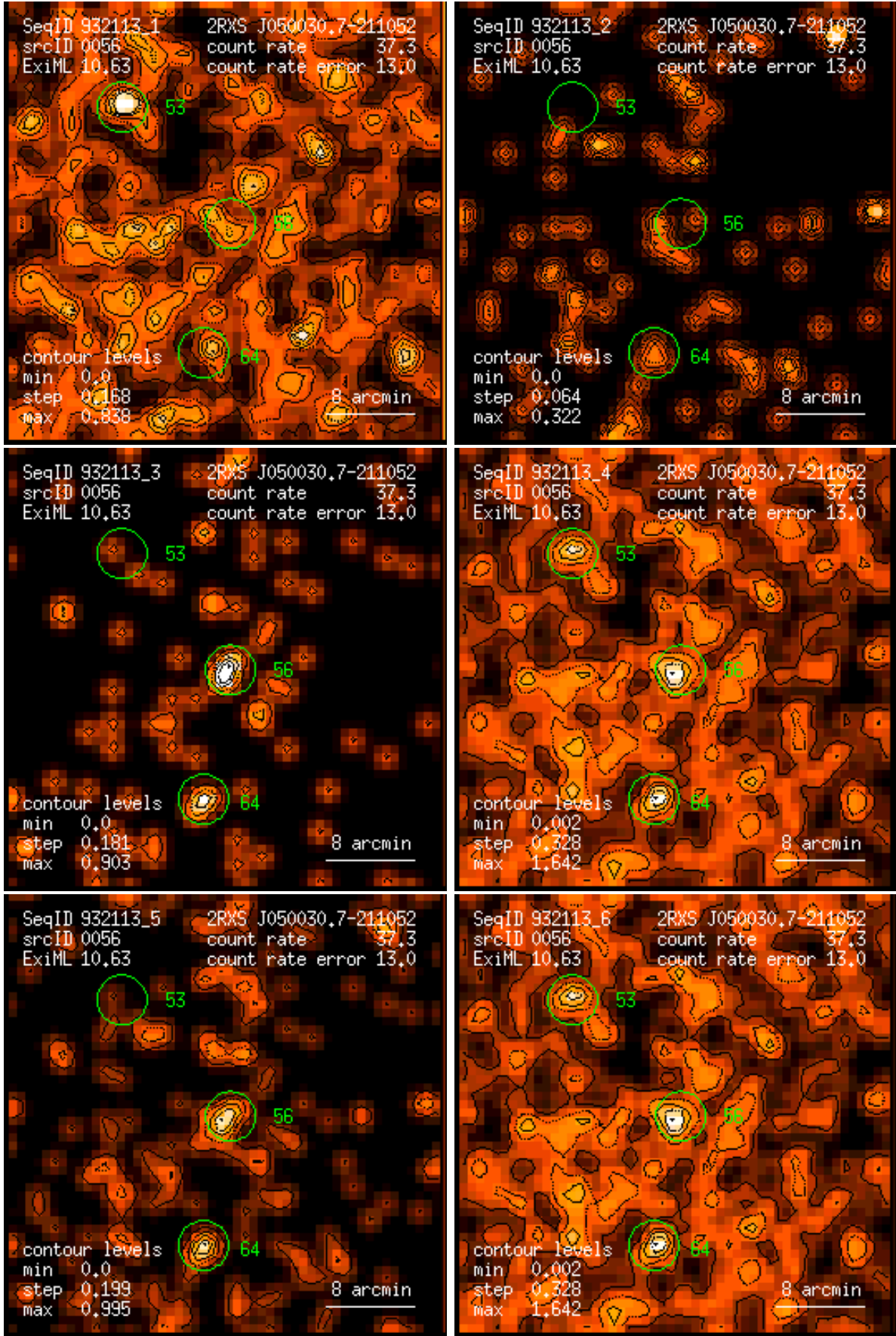
Figure 56: RASS 932113: detection 0056: band rate images, Gaussian filter: (1) PSPC channels 11 – 41, (2) 52 – 90, (3) 91 – 201, (4) 11 – 235, (5) 52 – 201, (6) 11 – 201. Broad band rates in counts/ks. Band rate contour levels in counts/ks/arcmin 2 .
