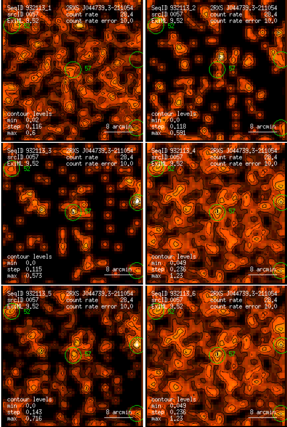
Figure 57: RASS 932113: detection 0057: band rate images, Gaussian filter: (1) PSPC channels 11 – 41, (2) 52 – 90, (3) 91 – 201, (4) 11 – 235, (5) 52 – 201, (6) 11 – 201. Broad band rates in counts/ks. Band rate contour levels in counts/ks/arcmin 2 .
