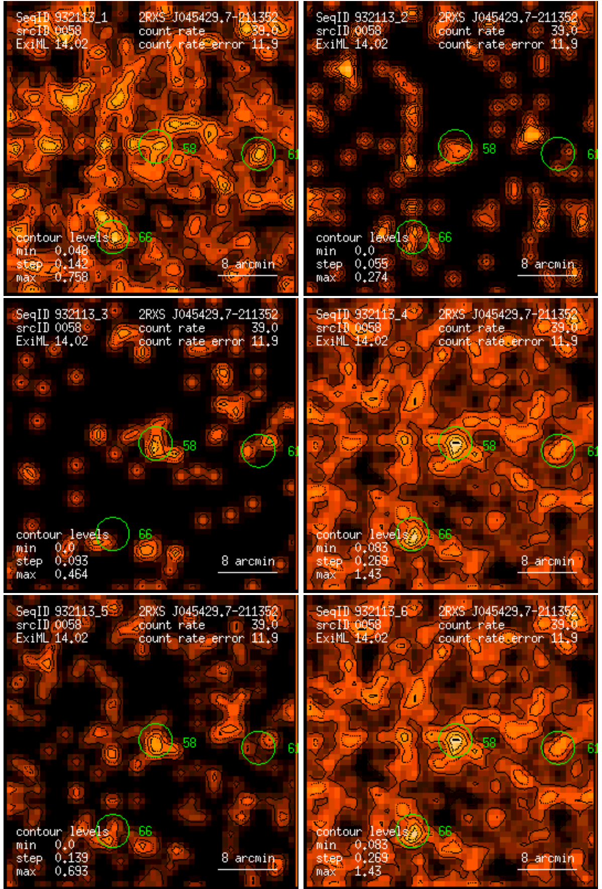
Figure 58: RASS 932113: detection 0058: band rate images, Gaussian filter: (1) PSPC channels 11 – 41, (2) 52 – 90, (3) 91 – 201, (4) 11 – 235, (5) 52 – 201, (6) 11 – 201. Broad band rates in counts/ks. Band rate contour levels in counts/ks/arcmin 2 .
