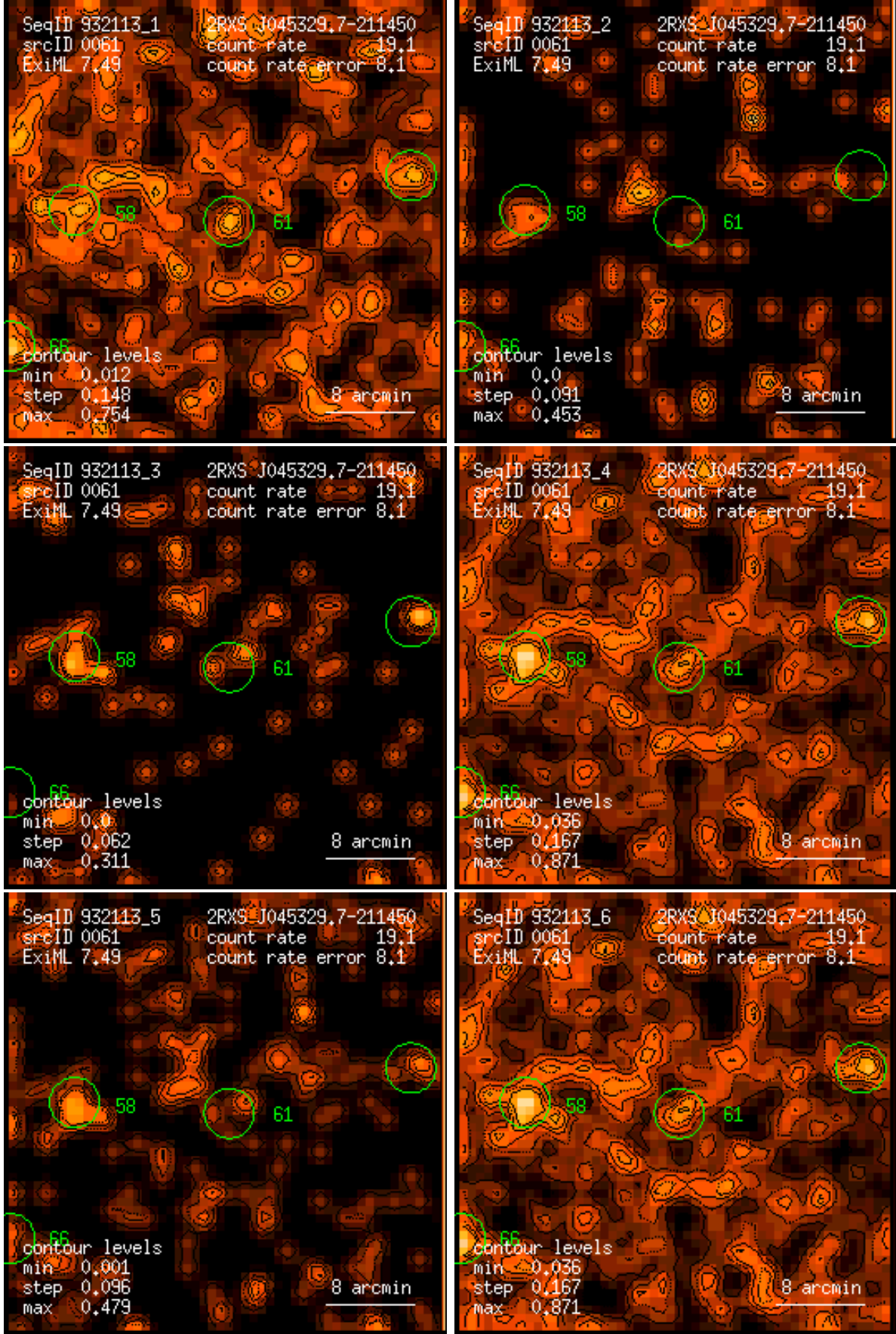
Figure 61: RASS 932113: detection 0061: band rate images, Gaussian filter: (1) PSPC channels 11 – 41, (2) 52 – 90, (3) 91 – 201, (4) 11 – 235, (5) 52 – 201, (6) 11 – 201. Broad band rates in counts/ks. Band rate contour levels in counts/ks/arcmin 2 .
