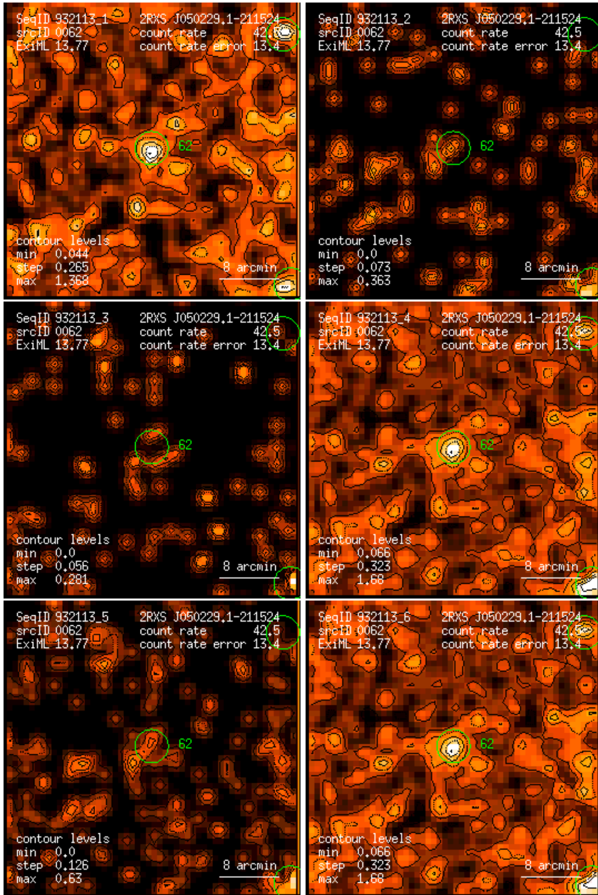
Figure 62: RASS 932113: detection 0062: band rate images, Gaussian filter: (1) PSPC channels 11 – 41, (2) 52 – 90, (3) 91 – 201, (4) 11 – 235, (5) 52 – 201, (6) 11 – 201. Broad band rates in counts/ks. Band rate contour levels in counts/ks/arcmin 2 .
