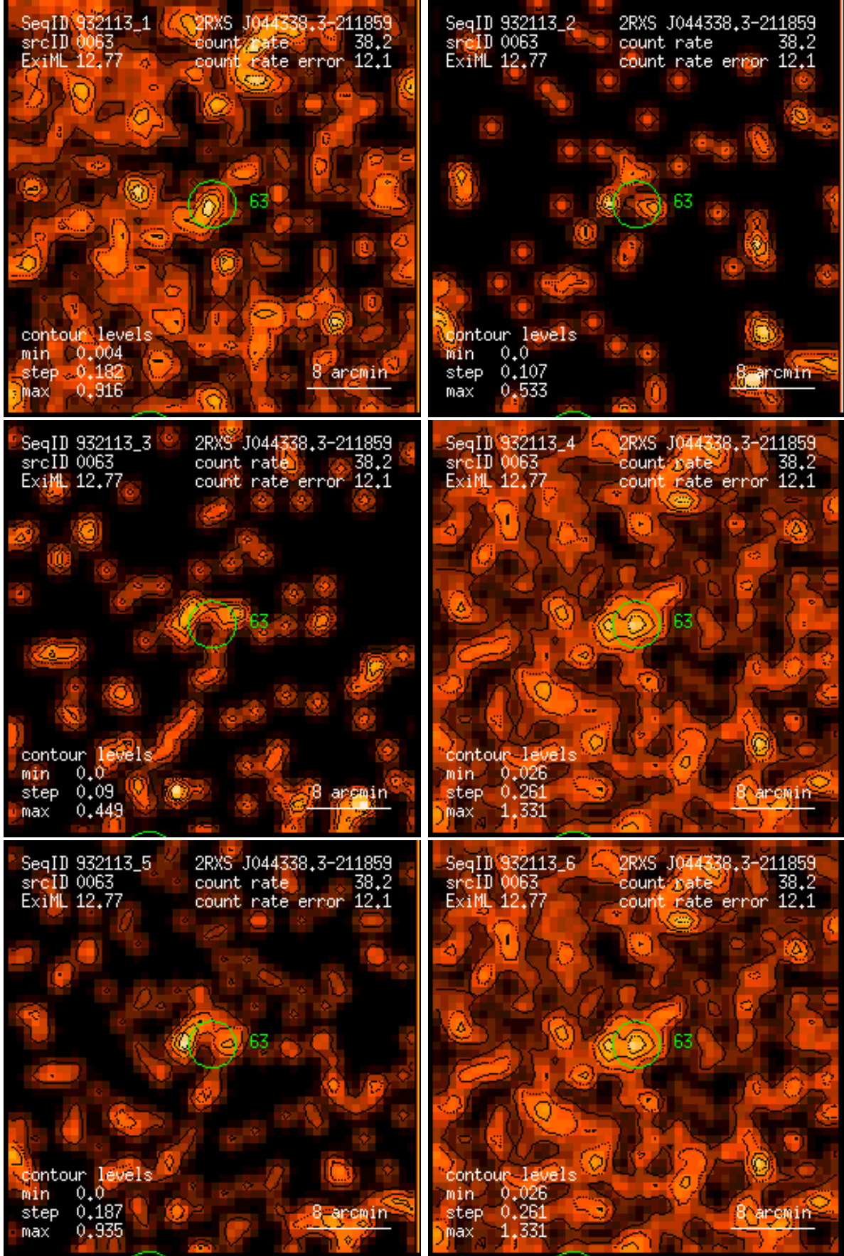
Figure 63: RASS 932113: detection 0063: band rate images, Gaussian filter: (1) PSPC channels 11 – 41, (2) 52 – 90, (3) 91 – 201, (4) 11 – 235, (5) 52 – 201, (6) 11 – 201. Broad band rates in counts/ks. Band rate contour levels in counts/ks/arcmin 2 .
