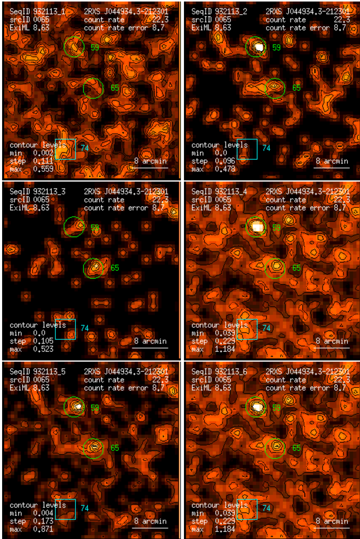
Figure 65: RASS 932113: detection 0065: band rate images, Gaussian filter: (1) PSPC channels 11 – 41, (2) 52 – 90, (3) 91 – 201, (4) 11 – 235, (5) 52 – 201, (6) 11 – 201. Broad band rates in counts/ks. Band rate contour levels in counts/ks/arcmin 2 .
