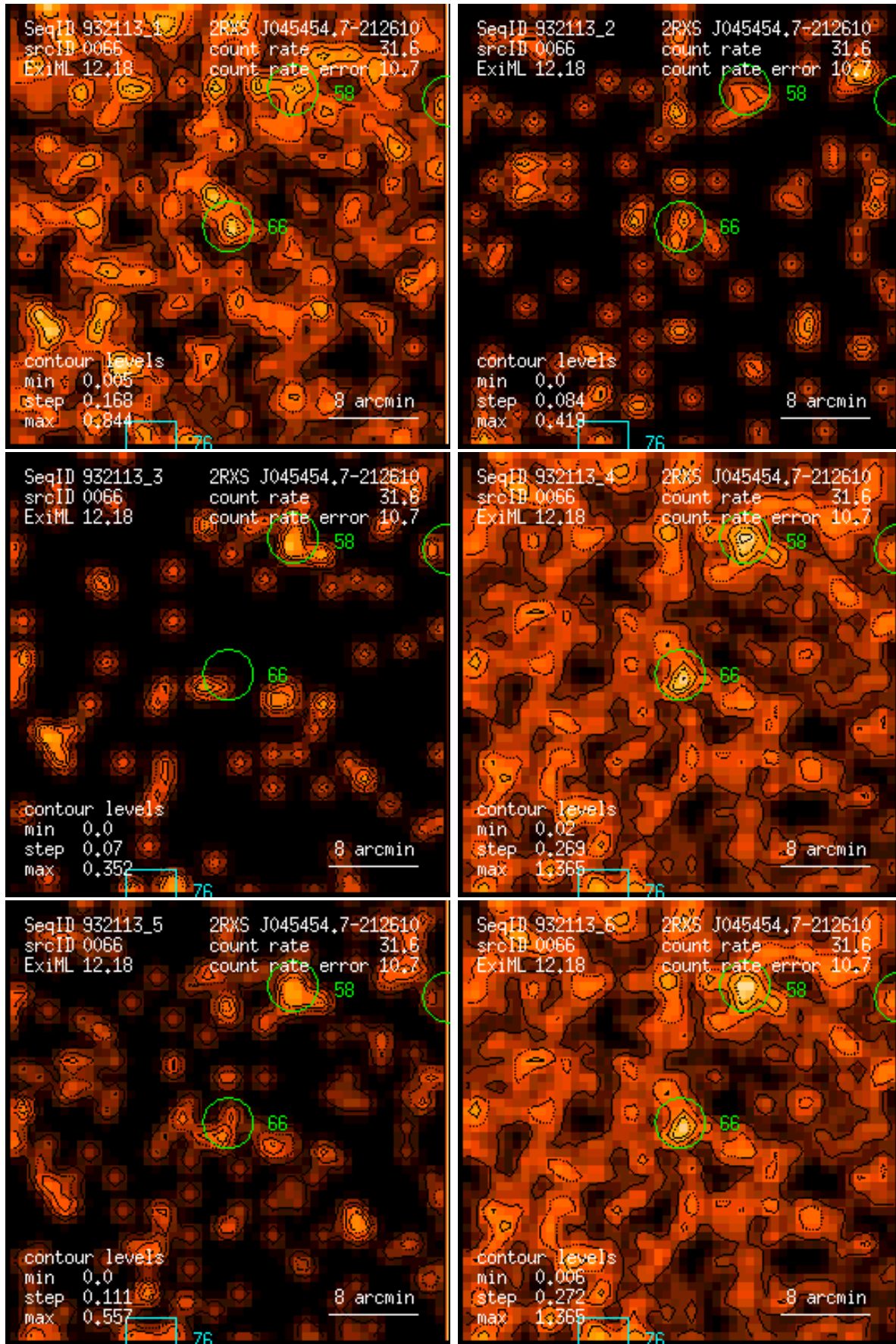
Figure 66: RASS 932113: detection 0066: band rate images, Gaussian filter: (1) PSPC channels 11 – 41, (2) 52 – 90, (3) 91 – 201, (4) 11 – 235, (5) 52 – 201, (6) 11 – 201. Broad band rates in counts/ks. Band rate contour levels in counts/ks/arcmin 2 .
