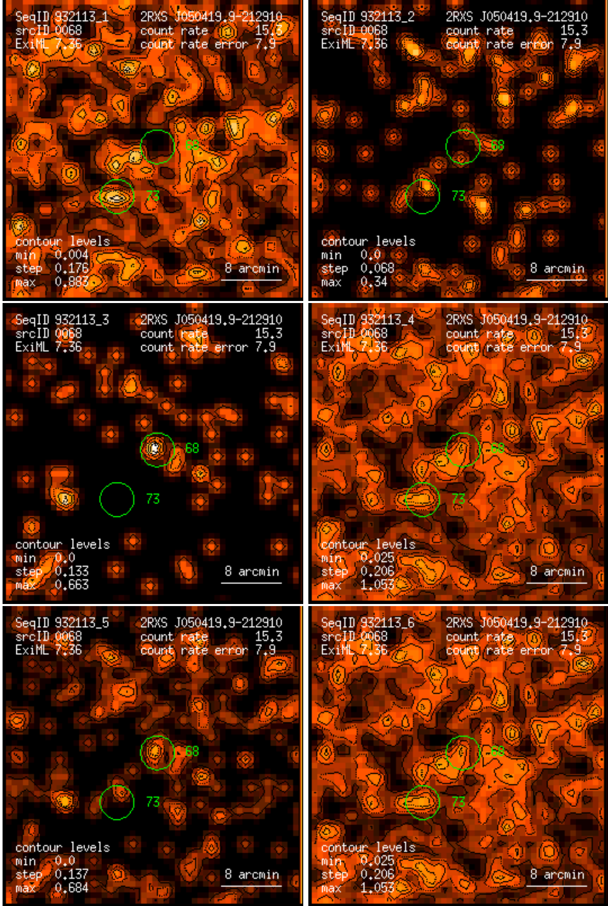
Figure 68: RASS 932113: detection 0068: band rate images, Gaussian filter: (1) PSPC channels 11 – 41, (2) 52 – 90, (3) 91 – 201, (4) 11 – 235, (5) 52 – 201, (6) 11 – 201. Broad band rates in counts/ks. Band rate contour levels in counts/ks/arcmin 2 .
