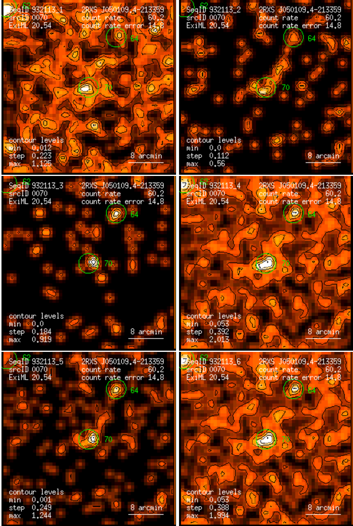
Figure 70: RASS 932113: detection 0070: band rate images, Gaussian filter: (1) PSPC channels 11 – 41, (2) 52 – 90, (3) 91 – 201, (4) 11 – 235, (5) 52 – 201, (6) 11 – 201. Broad band rates in counts/ks. Band rate contour levels in counts/ks/arcmin 2 .
